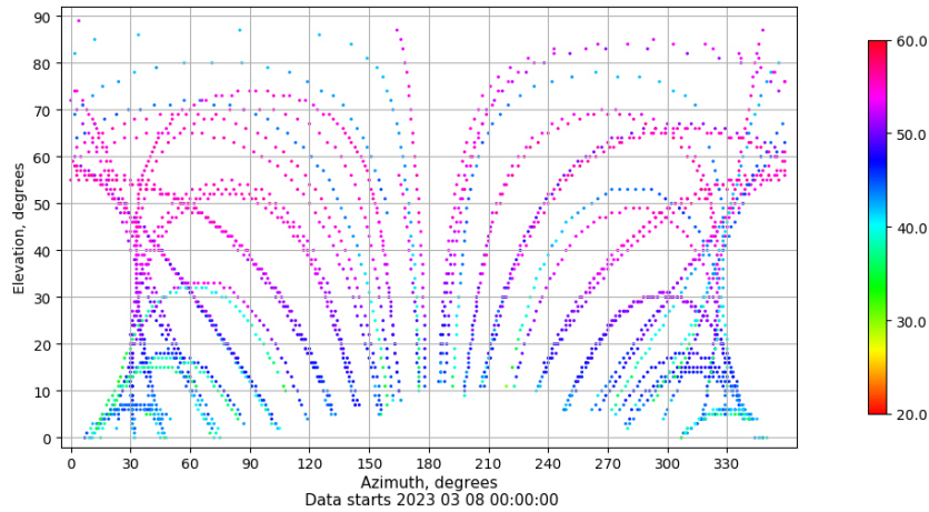
Azimuth-elevation plot for station SPAB. Signal to Noise S1C Data file SPAB00ESP_R_2023067.xtr
