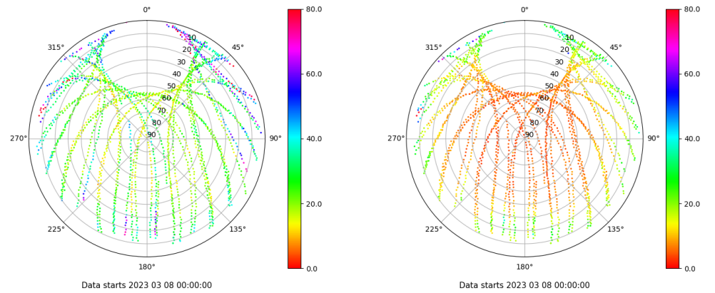
Skyplot for station SPAB. Parameter M1C Data file SPAB00ESP_R_2023067.xtr Skyplot for station SPAB. Parameter M2P Data file SPAB00ESP_R_2023067.xtr
