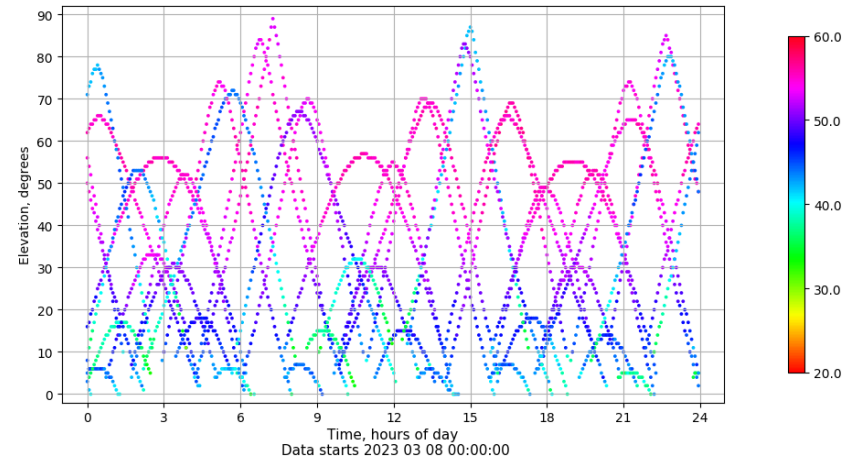
Time-elevation plot for station SPAB. Signal to Noise S1C Data file SPAB00ESP_R_2023067.xtr
