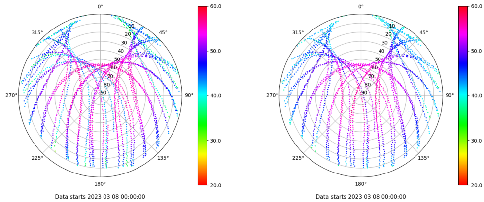
Skyplot for station SPAB. Signal to Noise S1C Data file SPAB00ESP_R_2023067.xtr Skyplot for station SPAB. Signal to Noise S2P Data file SPAB00ESP_R_2023067.xtr
