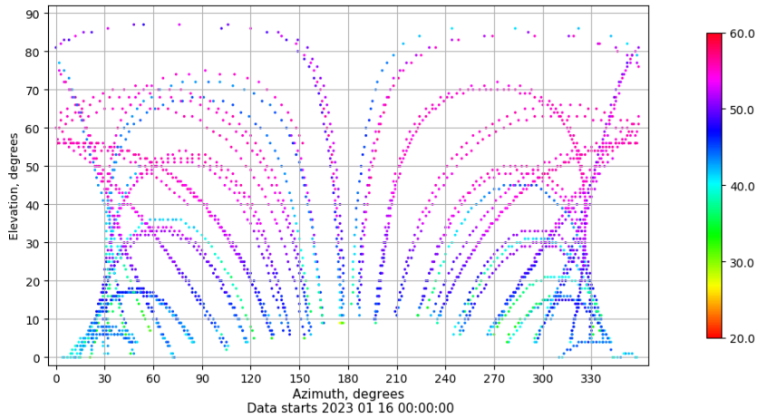
Azimuth-elevation plot for station SPAB. Signal to Noise S1C Data file SPAB00ESP_R_2023016.xtr
