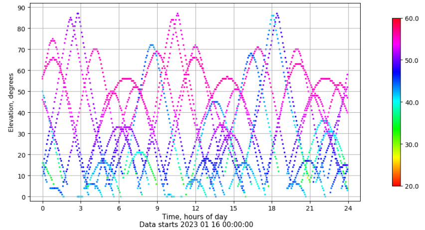
Time-elevation plot for station SPAB. Signal to Noise S1C Data file SPAB00ESP_R_2023016.xtr
