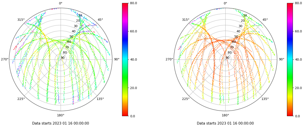
Skyplot for station SPAB. Parameter M1C Data file SPAB00ESP_R_2023016.xtr Skyplot for station SPAB. Parameter M2P Data file SPAB00ESP_R_2023016.xtr
