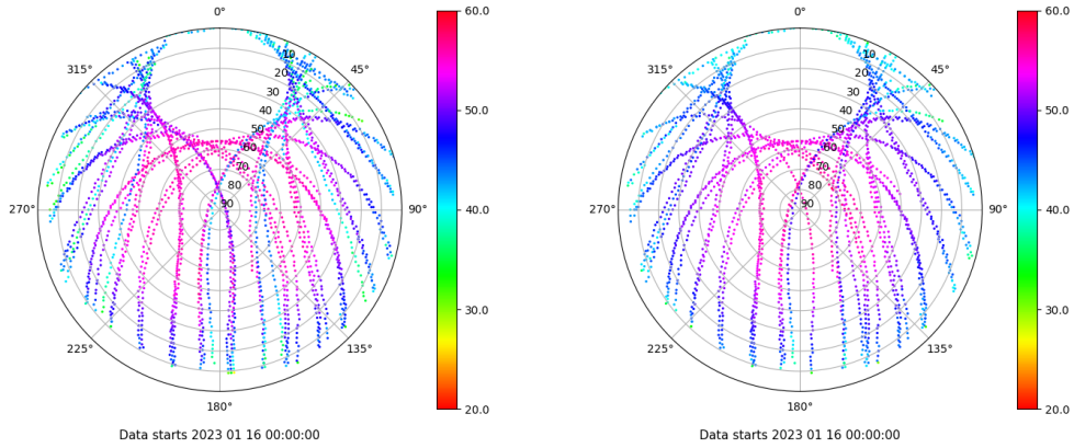
Skyplot for station SPAB. Signal to Noise S1C Data file SPAB00ESP_R_2023016.xtr Skyplot for station SPAB. Signal to Noise S2P Data file SPAB00ESP_R_2023016.xtr
