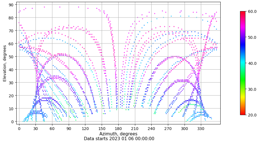
Azimuth-elevation plot for station SPAB. Signal to Noise S1C Data file SPAB00ESP_R_2023006.xtr
