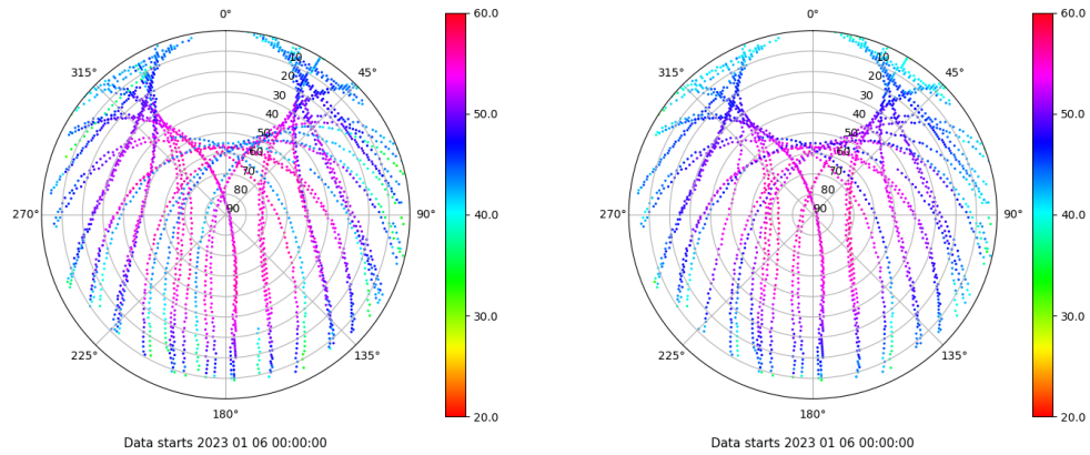
Skyplot for station SPAB. Signal to Noise S1C Data file SPAB00ESP_R_2023006.xtr Skyplot for station SPAB. Signal to Noise S2P Data file SPAB00ESP_R_2023006.xtr
