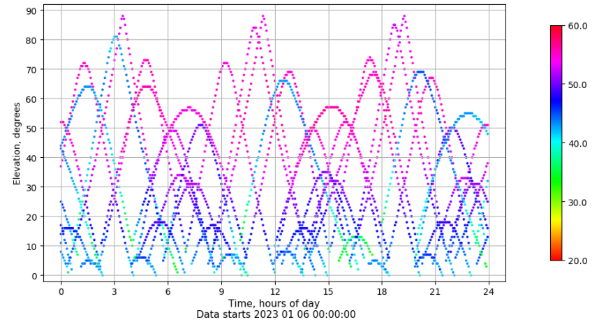
Time-elevation plot for station SPAB. Signal to Noise S1C Data file SPAB00ESP_R_2023006.xtr
