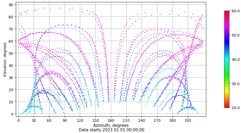
Azimuth-elevation plot for station SPAB. Signal to Noise S1C Data file SPAB00ESP_R_2023001.xtr
