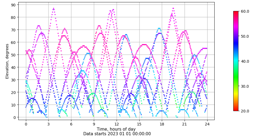
Time-elevation plot for station SPAB. Signal to Noise S1C Data file SPAB00ESP_R_2023001.xtr
