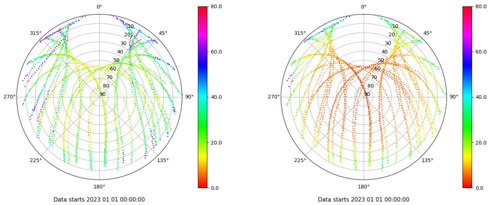
Skyplot for station SPAB. Parameter M1C Data file SPAB00ESP_R_2023001.xtr Skyplot for station SPAB. Parameter M2P Data file SPAB00ESP_R_2023001.xtr
