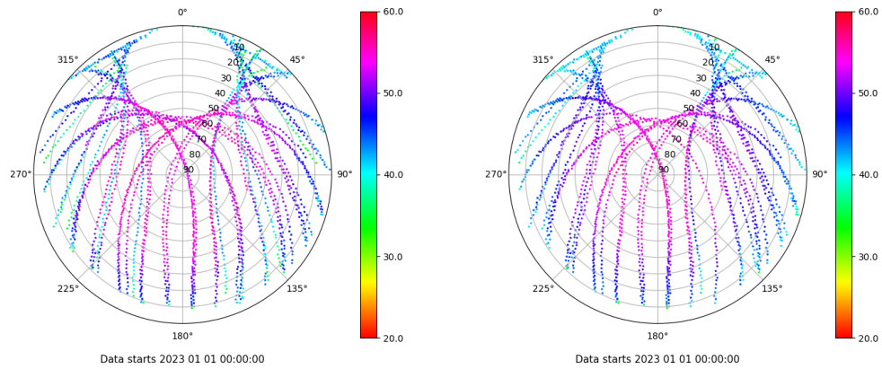
Skyplot for station SPAB. Signal to Noise S1C Data file SPAB00ESP_R_2023001.xtr Skyplot for station SPAB. Signal to Noise S2P Data file SPAB00ESP_R_2023001.xtr
