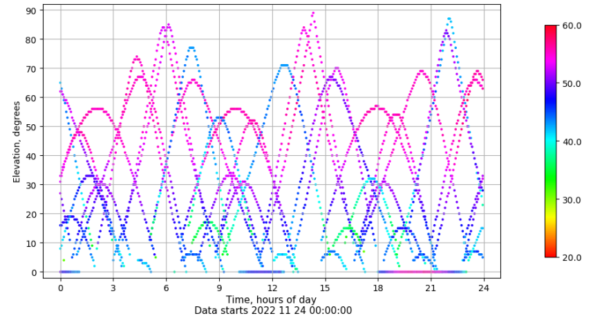
Time-elevation plot for station SPAB. Signal to Noise S1C Data file SPAB00ESP_R_2022328.xtr
