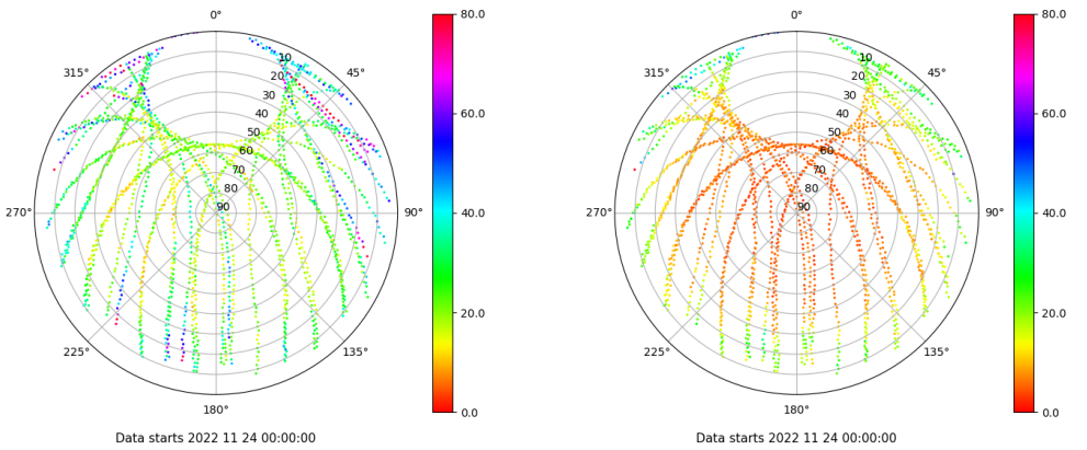
Skyplot for station SPAB. Parameter M1C Data file SPAB00ESP_R_2022328.xtr Skyplot for station SPAB. Parameter M2P Data file SPAB00ESP_R_2022328.xtr
