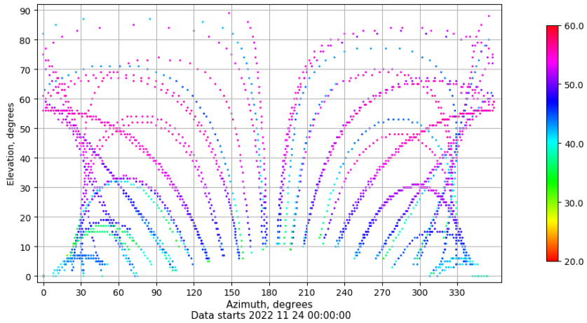
Azimuth-elevation plot for station SPAB. Signal to Noise S1C Data file SPAB00ESP_R_2022328.xtr
