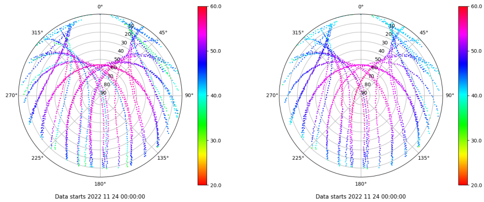
Skyplot for station SPAB. Signal to Noise S1C Data file SPAB00ESP_R_2022328.xtr Skyplot for station SPAB. Signal to Noise S2P Data file SPAB00ESP_R_2022328.xtr
