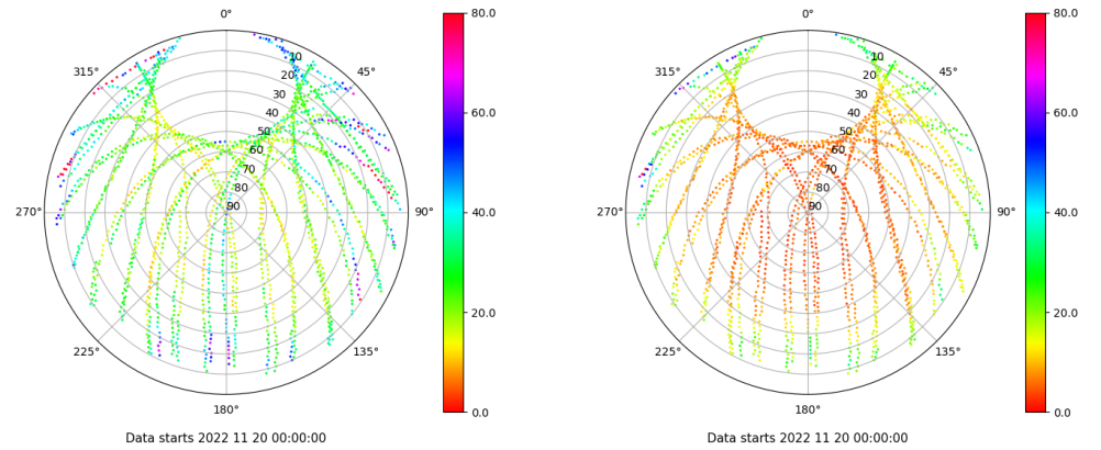
Skyplot for station SPAB. Parameter M1C Data file SPAB00ESP_R_2022324.xtr Skyplot for station SPAB. Parameter M2P Data file SPAB00ESP_R_2022324.xtr
