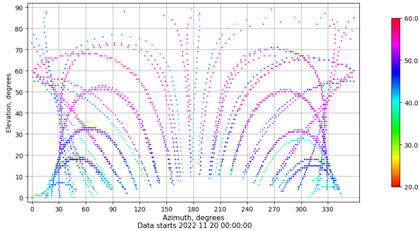
Azimuth-elevation plot for station SPAB. Signal to Noise S1C Data file SPAB00ESP_R_2022324.xtr
