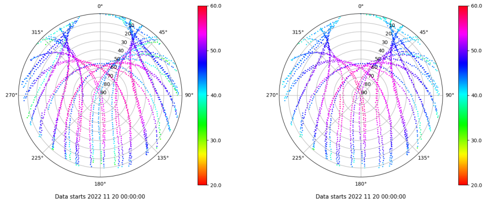
Skyplot for station SPAB. Signal to Noise S1C Data file SPAB00ESP_R_2022324.xtr Skyplot for station SPAB. Signal to Noise S2P Data file SPAB00ESP_R_2022324.xtr
