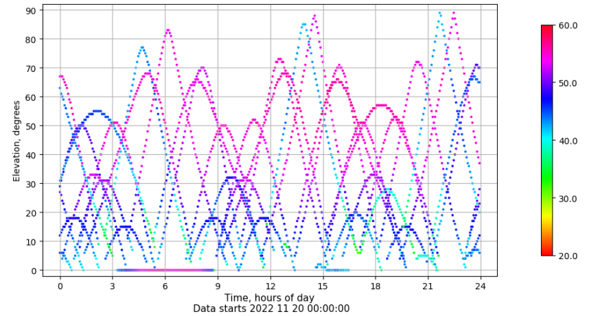
Time-elevation plot for station SPAB. Signal to Noise S1C Data file SPAB00ESP_R_2022324.xtr
