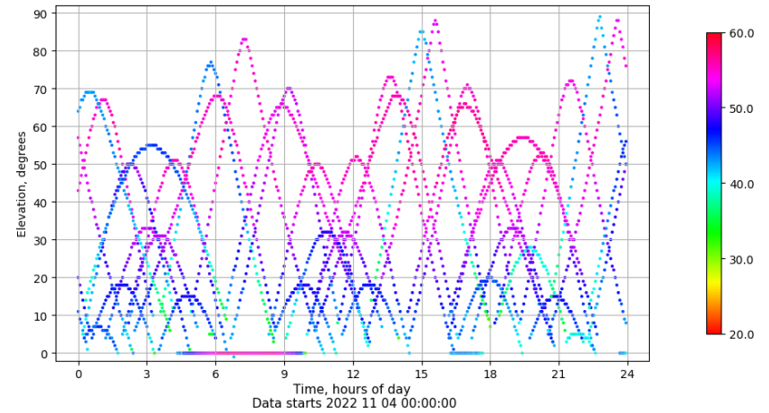
Time-elevation plot for station SPAB. Signal to Noise S1C Data file SPAB00ESP_R_2022308.xtr
