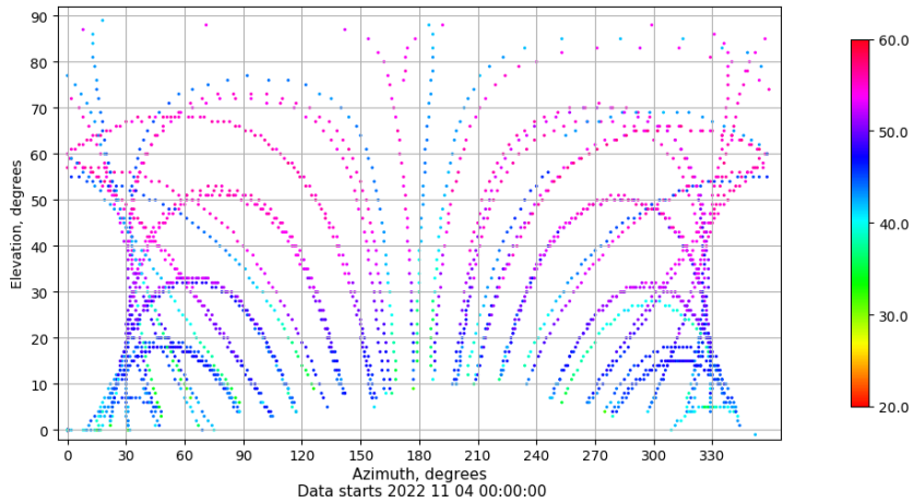
Azimuth-elevation plot for station SPAB. Signal to Noise S1C Data file SPAB00ESP_R_2022308.xtr
