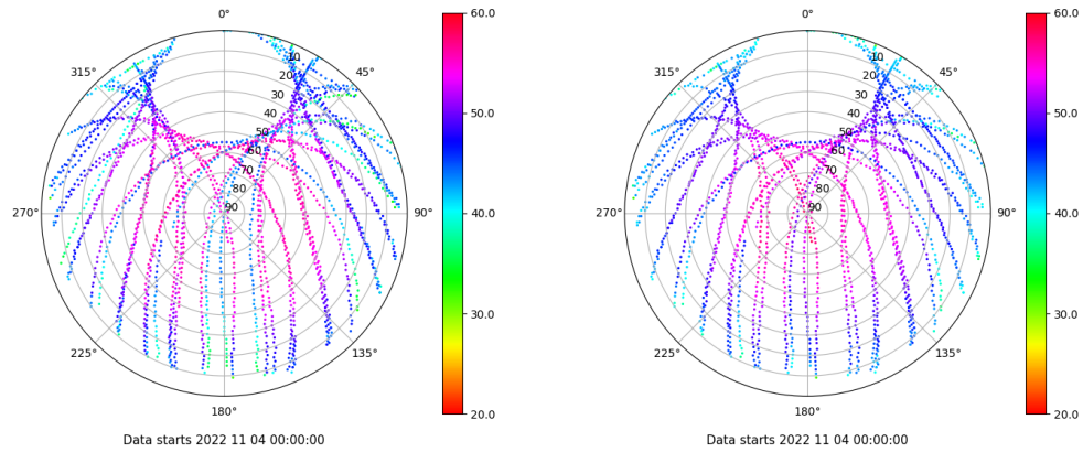
Skyplot for station SPAB. Signal to Noise S1C Data file SPAB00ESP_R_2022308.xtr Skyplot for station SPAB. Signal to Noise S2P Data file SPAB00ESP_R_2022308.xtr
