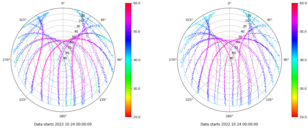
Skyplot for station SPAB. Signal to Noise S1C Data file SPAB00ESP_R_2022297.xtr Skyplot for station SPAB. Signal to Noise S2P Data file SPAB00ESP_R_2022297.xtr
