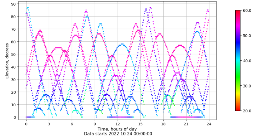
Time-elevation plot for station SPAB. Signal to Noise S1C Data file SPAB00ESP_R_2022297.xtr
