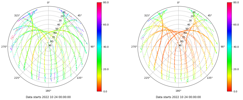
Skyplot for station SPAB. Parameter M1C Data file SPAB00ESP_R_2022297.xtr Skyplot for station SPAB. Parameter M2P Data file SPAB00ESP_R_2022297.xtr
