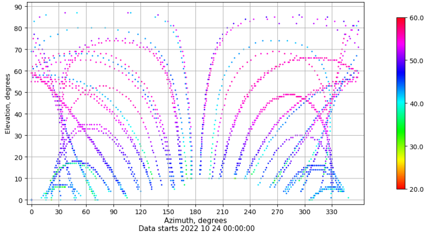
Azimuth-elevation plot for station SPAB. Signal to Noise S1C Data file SPAB00ESP_R_2022297.xtr
