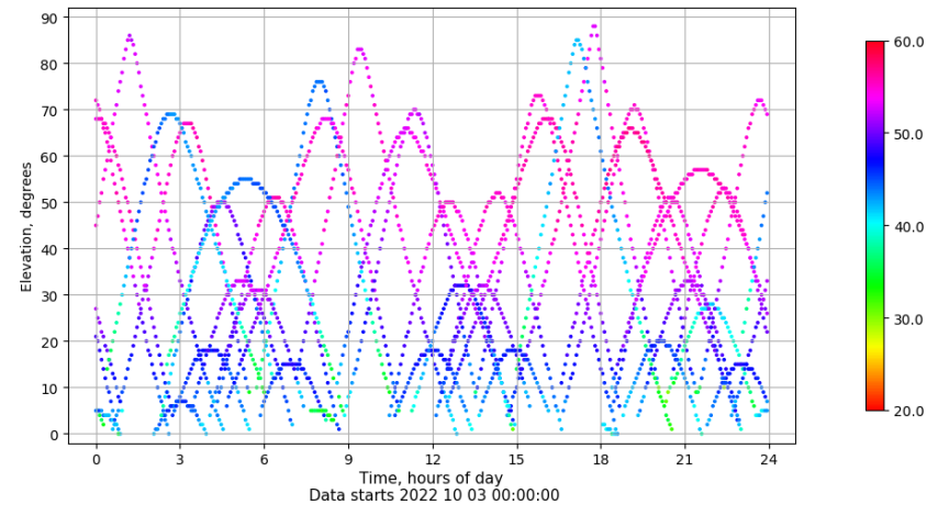
Time-elevation plot for station SPAB. Signal to Noise S1C Data file SPAB00ESP_R_2022276.xtr
