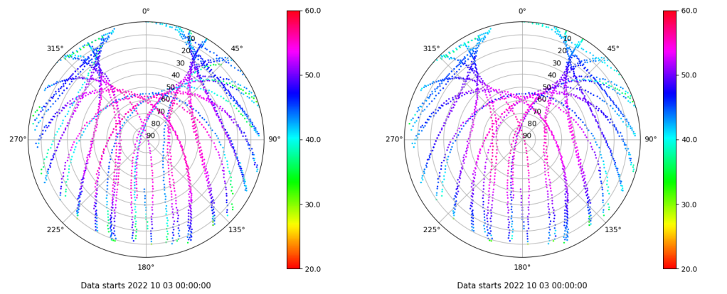
Skyplot for station SPAB. Signal to Noise S1C Data file SPAB00ESP_R_2022276.xtr Skyplot for station SPAB. Signal to Noise S2P Data file SPAB00ESP_R_2022276.xtr
