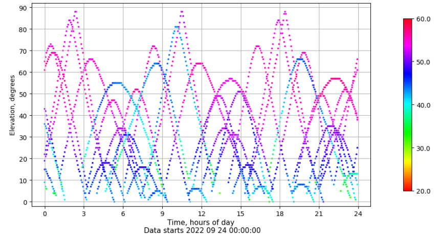
Time-elevation plot for station SPAB. Signal to Noise S1C Data file SPAB00ESP_R_2022267.xtr
