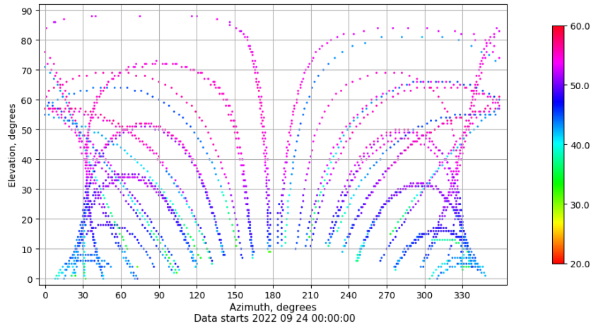
Azimuth-elevation plot for station SPAB. Signal to Noise S1C Data file SPAB00ESP_R_2022267.xtr
