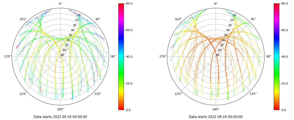
Skyplot for station SPAB. Parameter M1C Data file SPAB00ESP_R_2022267.xtr Skyplot for station SPAB. Parameter M2P Data file SPAB00ESP_R_2022267.xtr
