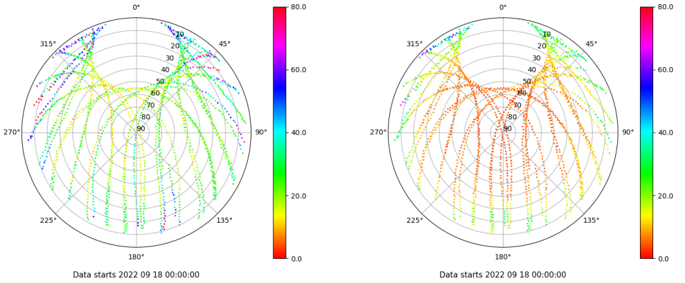
Skyplot for station SPAB. Parameter M1C Data file SPAB00ESP_R_2022261.xtr Skyplot for station SPAB. Parameter M2P Data file SPAB00ESP_R_2022261.xtr
