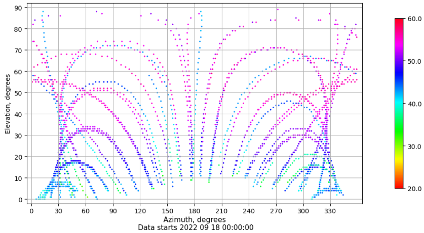
Azimuth-elevation plot for station SPAB. Signal to Noise S1C Data file SPAB00ESP_R_2022261.xtr
