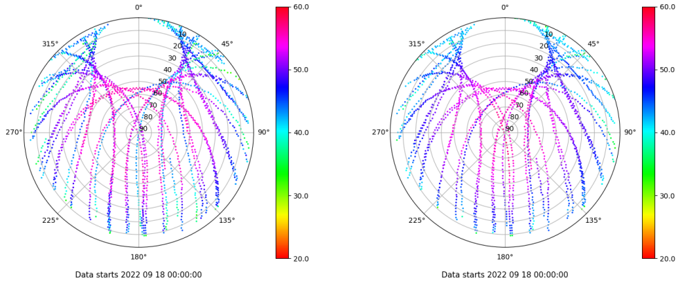
Skyplot for station SPAB. Signal to Noise S1C Data file SPAB00ESP_R_2022261.xtr Skyplot for station SPAB. Signal to Noise S2P Data file SPAB00ESP_R_2022261.xtr
