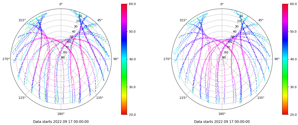
Skyplot for station SPAB. Signal to Noise S1C Data file SPAB00ESP_R_2022260.xtr Skyplot for station SPAB. Signal to Noise S2P Data file SPAB00ESP_R_2022260.xtr
