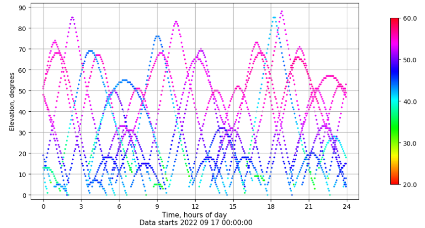
Time-elevation plot for station SPAB. Signal to Noise S1C Data file SPAB00ESP_R_2022260.xtr
