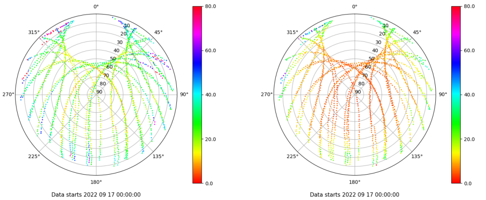
Skyplot for station SPAB. Parameter M1C Data file SPAB00ESP_R_2022260.xtr Skyplot for station SPAB. Parameter M2P Data file SPAB00ESP_R_2022260.xtr
