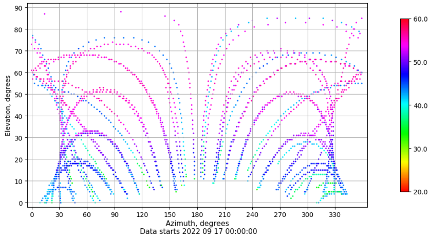
Azimuth-elevation plot for station SPAB. Signal to Noise S1C Data file SPAB00ESP_R_2022260.xtr
