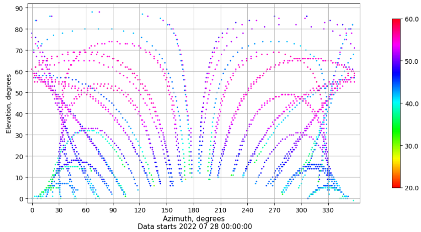
Azimuth-elevation plot for station SPAB. Signal to Noise S1C Data file SPAB00ESP_R_2022209.xtr
