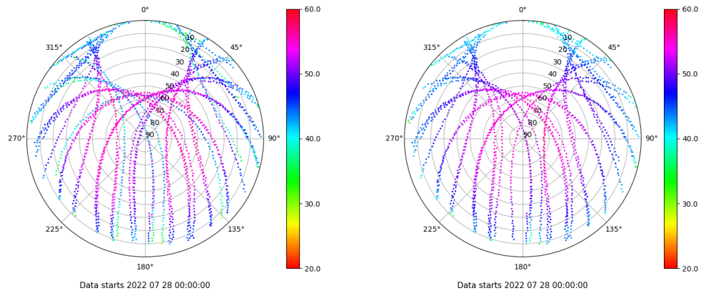
Skyplot for station SPAB. Signal to Noise S1C Data file SPAB00ESP_R_2022209.xtr Skyplot for station SPAB. Signal to Noise S2P Data file SPAB00ESP_R_2022209.xtr
