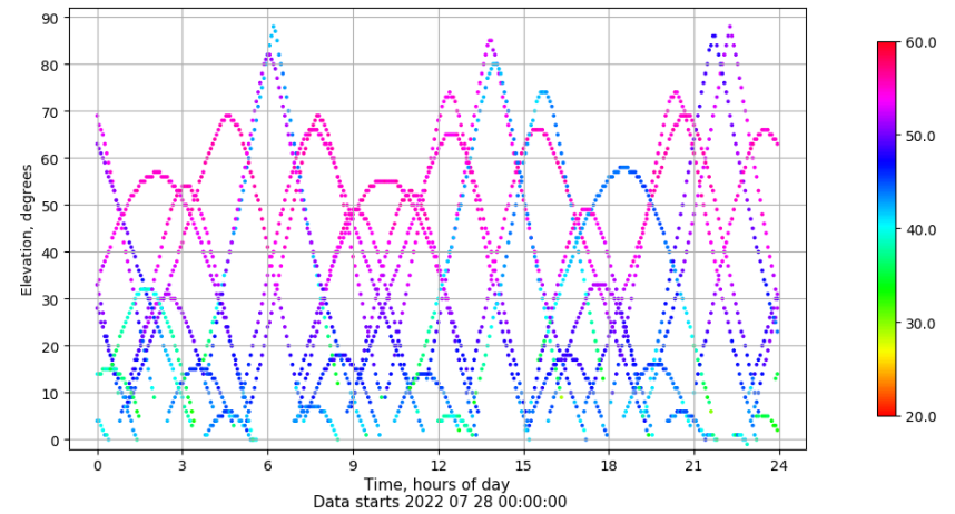
Time-elevation plot for station SPAB. Signal to Noise S1C Data file SPAB00ESP_R_2022209.xtr
