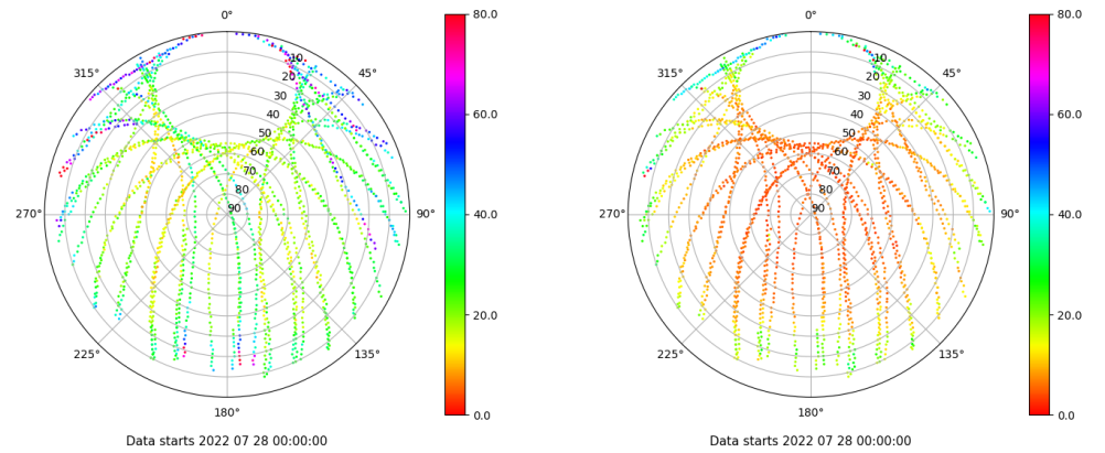
Skyplot for station SPAB. Parameter M1C Data file SPAB00ESP_R_2022209.xtr Skyplot for station SPAB. Parameter M2P Data file SPAB00ESP_R_2022209.xtr
