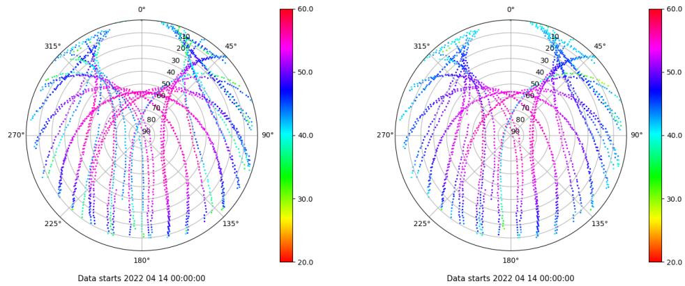
Skyplot for station SPAB. Signal to Noise S1C Data file SPAB00ESP_R_2022104.xtr Skyplot for station SPAB. Signal to Noise S2P Data file SPAB00ESP_R_2022104.xtr
