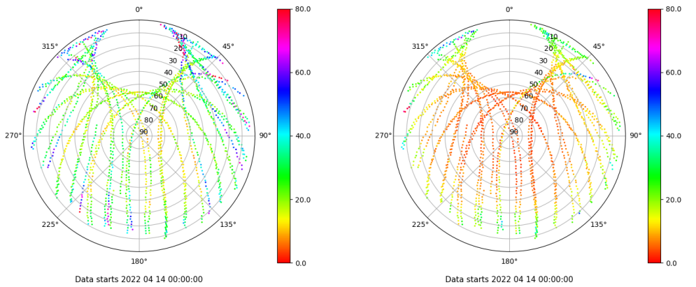
Skyplot for station SPAB. Parameter M1C Data file SPAB00ESP_R_2022104.xtr Skyplot for station SPAB. Parameter M2P Data file SPAB00ESP_R_2022104.xtr
