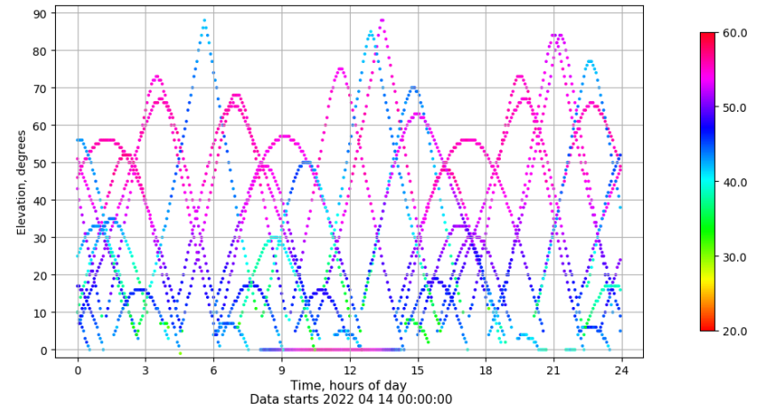
Time-elevation plot for station SPAB. Signal to Noise S1C Data file SPAB00ESP_R_2022104.xtr
