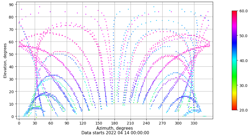
Azimuth-elevation plot for station SPAB. Signal to Noise S1C Data file SPAB00ESP_R_2022104.xtr
