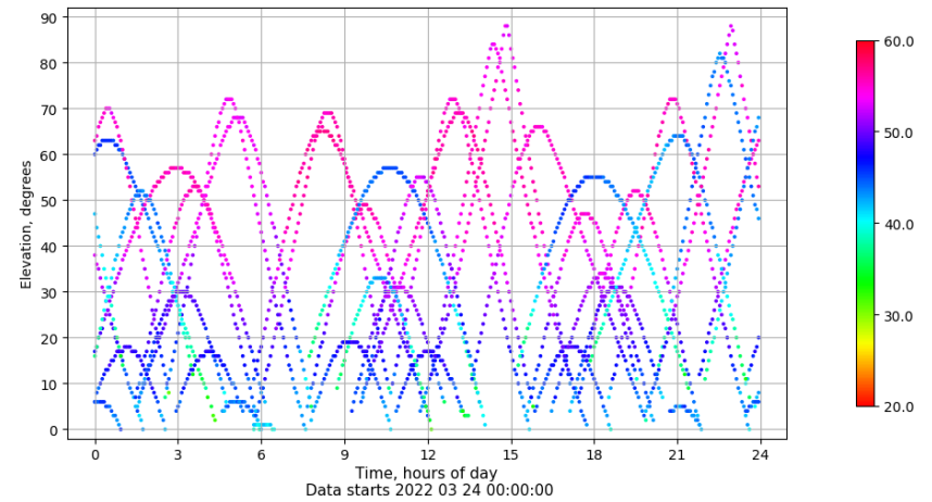
Time-elevation plot for station SPAB. Signal to Noise S1C Data file SPAB00ESP_R_2022083.xtr
