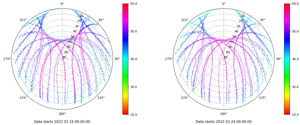
Skyplot for station SPAB. Signal to Noise S1C Data file SPAB00ESP_R_2022083.xtr Skyplot for station SPAB. Signal to Noise S2P Data file SPAB00ESP_R_2022083.xtr
