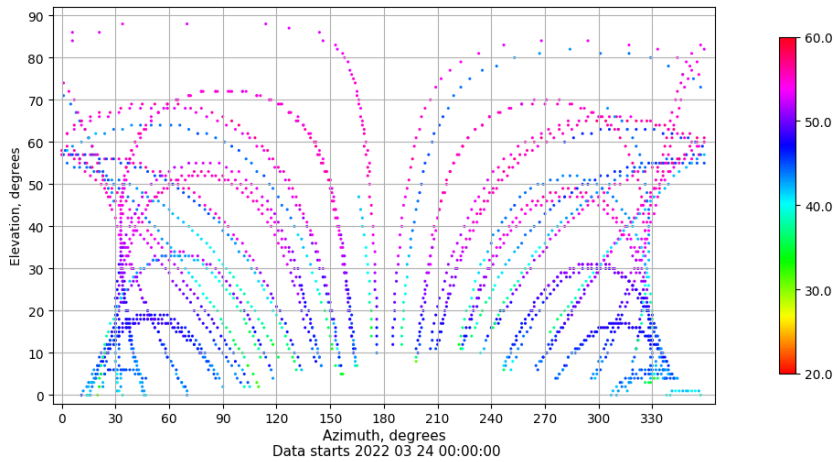
Azimuth-elevation plot for station SPAB. Signal to Noise S1C Data file SPAB00ESP_R_2022083.xtr
