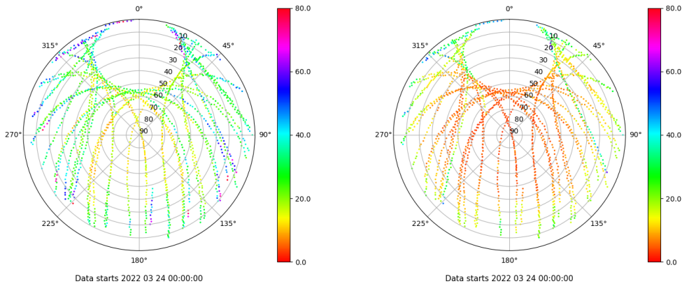
Skyplot for station SPAB. Parameter M1C Data file SPAB00ESP_R_2022083.xtr Skyplot for station SPAB. Parameter M2P Data file SPAB00ESP_R_2022083.xtr
