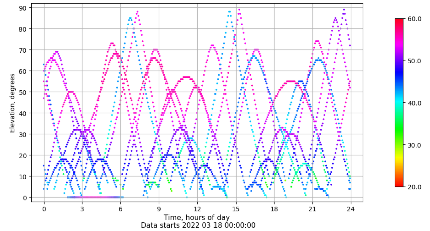
Time-elevation plot for station SPAB. Signal to Noise S1C Data file SPAB00ESP_R_2022077.xtr
