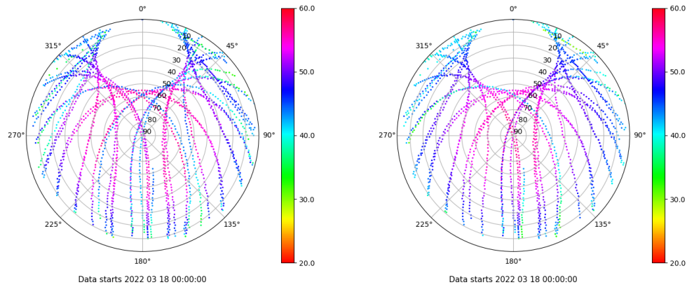
Skyplot for station SPAB. Signal to Noise S1C Data file SPAB00ESP_R_2022077.xtr Skyplot for station SPAB. Signal to Noise S2P Data file SPAB00ESP_R_2022077.xtr
