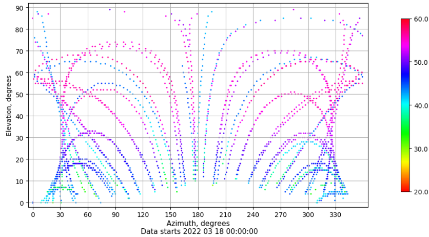
Azimuth-elevation plot for station SPAB. Signal to Noise S1C Data file SPAB00ESP_R_2022077.xtr
