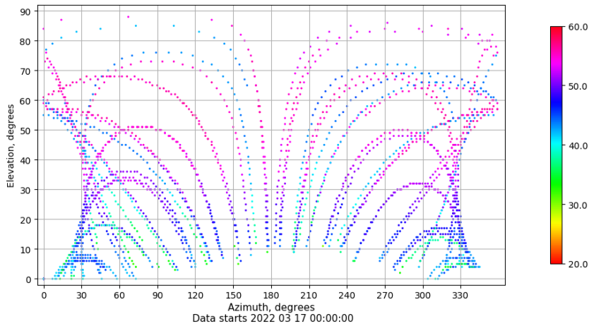
Azimuth-elevation plot for station SPAB. Signal to Noise S1C Data file SPAB00ESP_R_2022076.xtr
