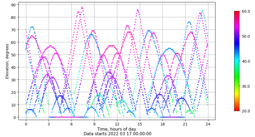
Time-elevation plot for station SPAB. Signal to Noise S1C Data file SPAB00ESP_R_2022076.xtr
