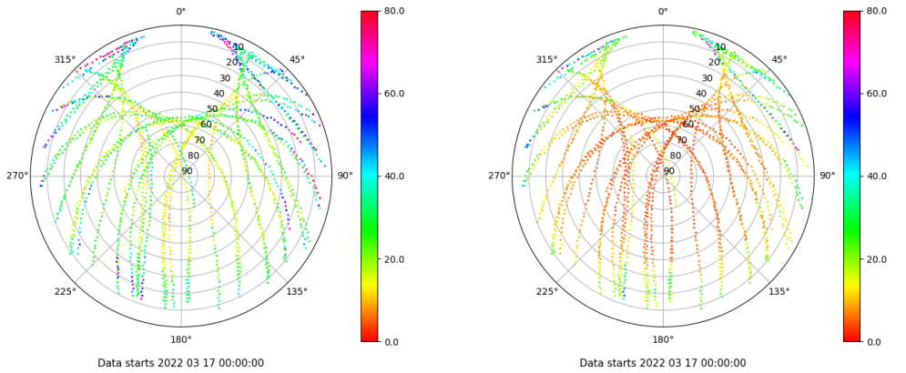
Skyplot for station SPAB. Parameter M1C Data file SPAB00ESP_R_2022076.xtr Skyplot for station SPAB. Parameter M2P Data file SPAB00ESP_R_2022076.xtr
