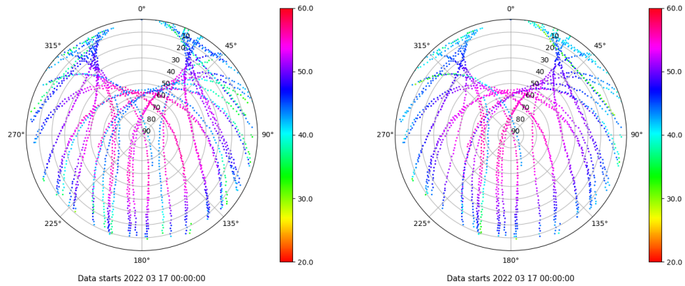
Skyplot for station SPAB. Signal to Noise S1C Data file SPAB00ESP_R_2022076.xtr Skyplot for station SPAB. Signal to Noise S2P Data file SPAB00ESP_R_2022076.xtr
