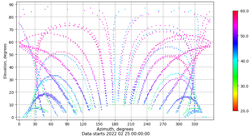
Azimuth-elevation plot for station SPAB. Signal to Noise S1C Data file SPAB00ESP_R_2022056.xtr
