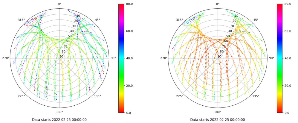
Skyplot for station SPAB. Parameter M1C Data file SPAB00ESP_R_2022056.xtr Skyplot for station SPAB. Parameter M2P Data file SPAB00ESP_R_2022056.xtr
