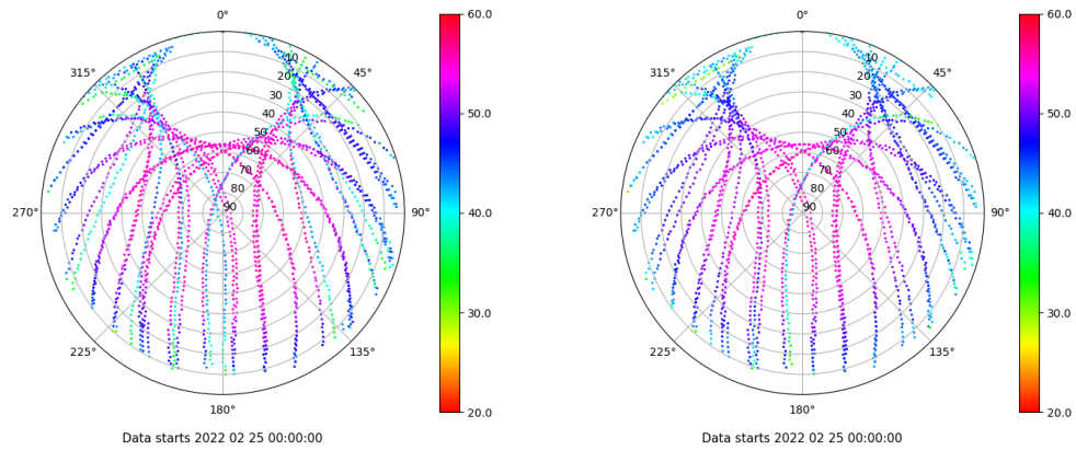
Skyplot for station SPAB. Signal to Noise S1C Data file SPAB00ESP_R_2022056.xtr Skyplot for station SPAB. Signal to Noise S2P Data file SPAB00ESP_R_2022056.xtr
