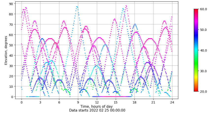
Time-elevation plot for station SPAB. Signal to Noise S1C Data file SPAB00ESP_R_2022056.xtr
