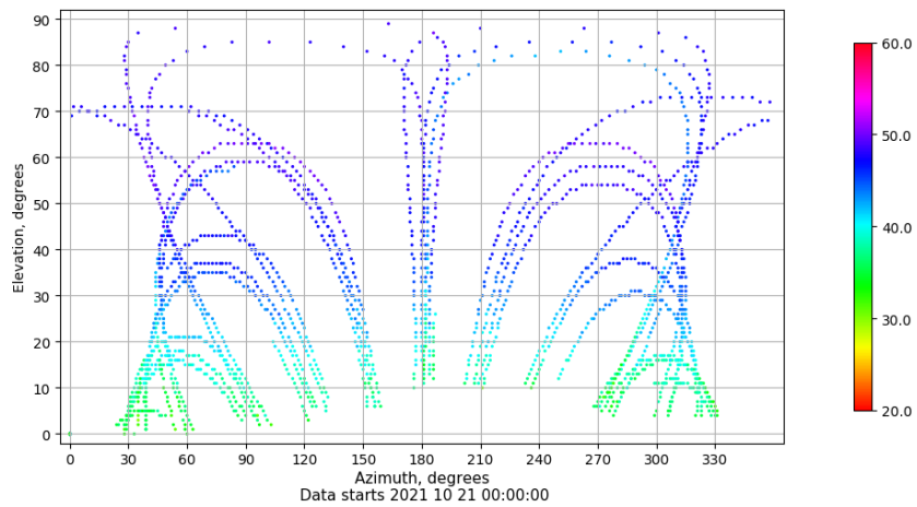
Azimuth-elevation plot for station SPAB. Signal to Noise S1X Data file SPAB00ESP_R_2021294.xtr
