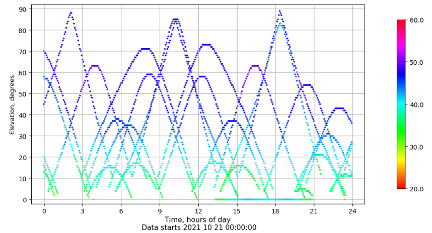
Time-elevation plot for station SPAB. Signal to Noise S1X Data file SPAB00ESP_R_2021294.xtr
