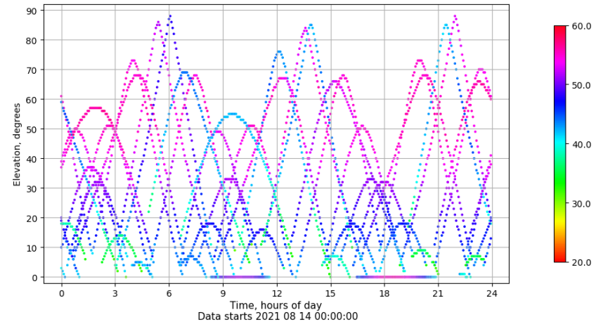
Time-elevation plot for station SPAB. Signal to Noise S1C Data file SPAB00ESP_R_2021226.xtr
