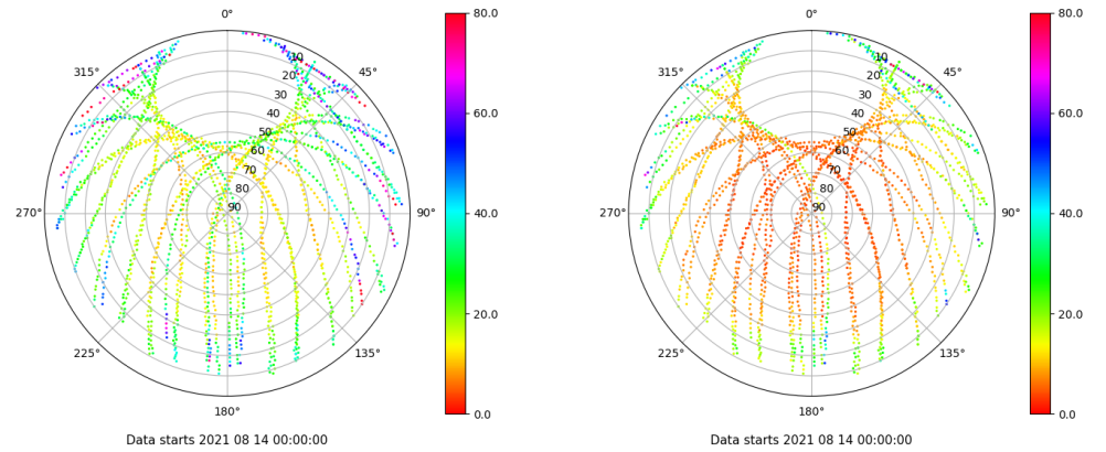
Skyplot for station SPAB. Parameter M1C Data file SPAB00ESP_R_2021226.xtr Skyplot for station SPAB. Parameter M2P Data file SPAB00ESP_R_2021226.xtr
