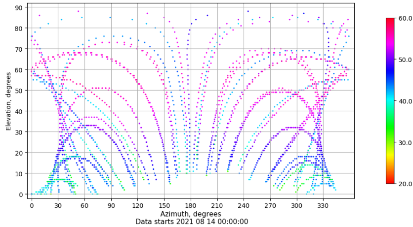
Azimuth-elevation plot for station SPAB. Signal to Noise S1C Data file SPAB00ESP_R_2021226.xtr
