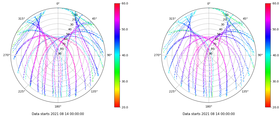
Skyplot for station SPAB. Signal to Noise S1C Data file SPAB00ESP_R_2021226.xtr Skyplot for station SPAB. Signal to Noise S2P Data file SPAB00ESP_R_2021226.xtr
