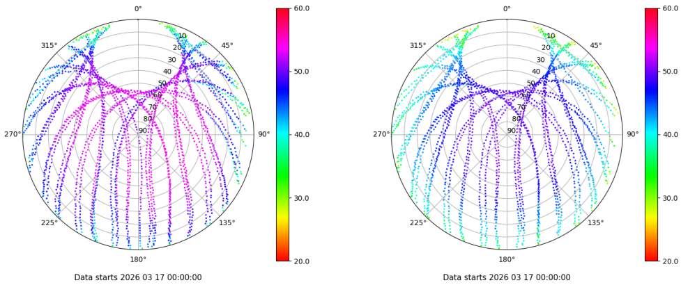
Skyplot for station SINE. Signal to Noise S1C Data file SINE00ESP_R_2026076.xtr Skyplot for station SINE. Signal to Noise S2P Data file SINE00ESP_R_2026076.xtr
