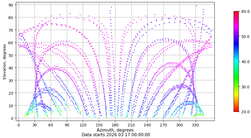
Azimuth-elevation plot for station SINE. Signal to Noise S1C Data file SINE00ESP_R_2026076.xtr
