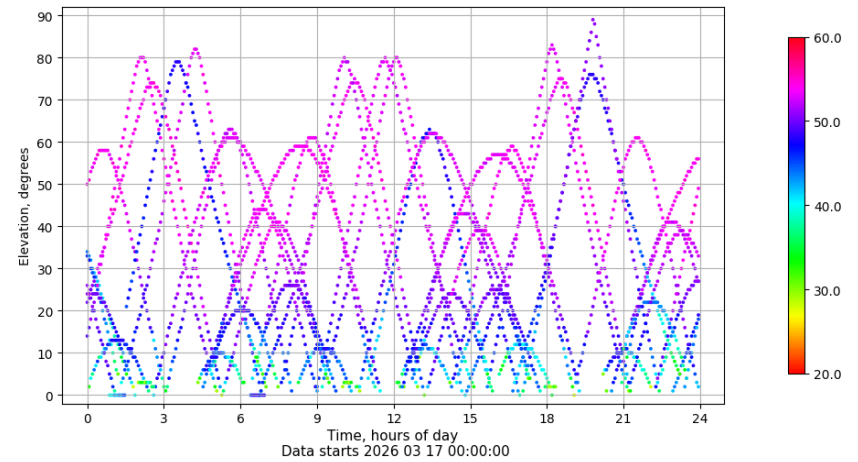
Time-elevation plot for station SINE. Signal to Noise S1C Data file SINE00ESP_R_2026076.xtr
