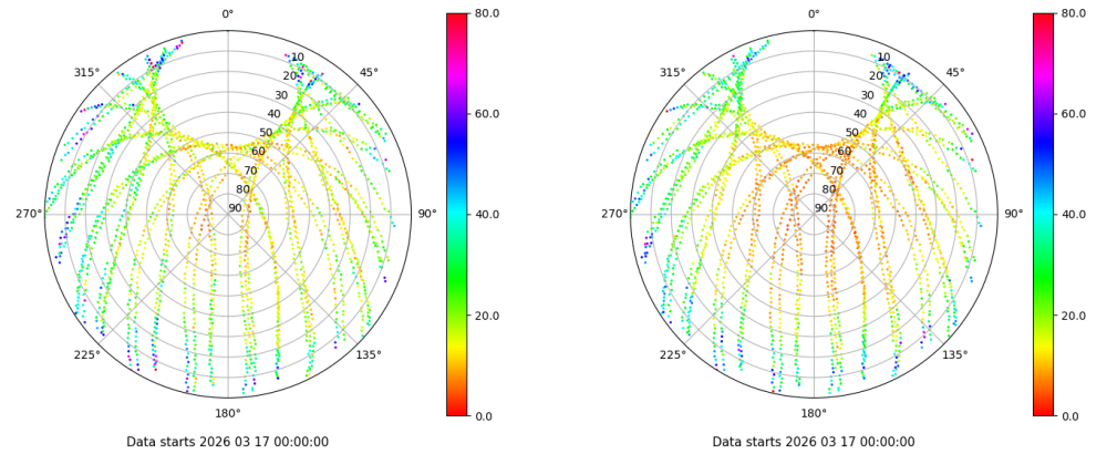
Skyplot for station SINE. Parameter M1C Data file SINE00ESP_R_2026076.xtr Skyplot for station SINE. Parameter M2P Data file SINE00ESP_R_2026076.xtr
