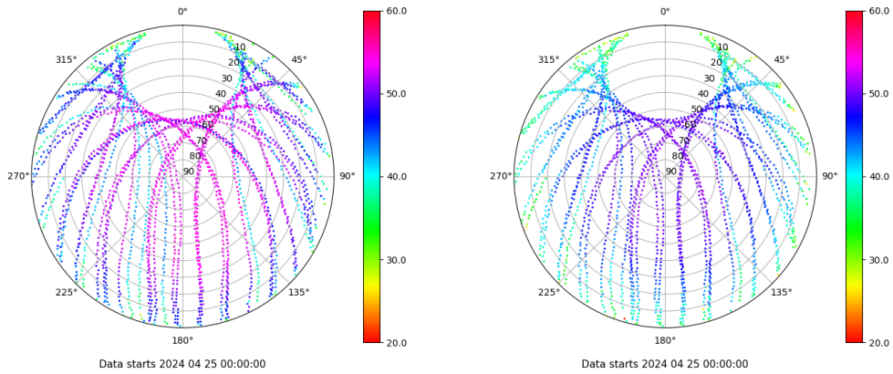
Skyplot for station SINE. Signal to Noise S1C Data file SINE00ESP_R_2024116.xtr Skyplot for station SINE. Signal to Noise S2P Data file SINE00ESP_R_2024116.xtr
