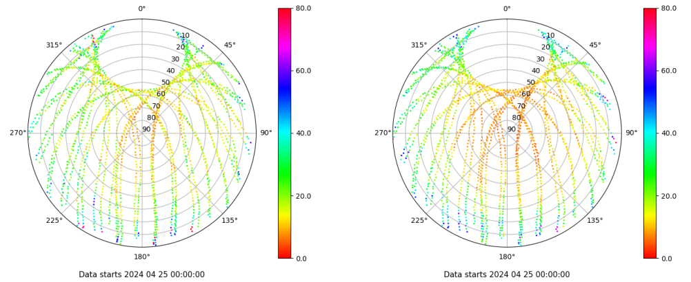
Skyplot for station SINE. Parameter M1C Data file SINE00ESP_R_2024116.xtr Skyplot for station SINE. Parameter M2P Data file SINE00ESP_R_2024116.xtr
