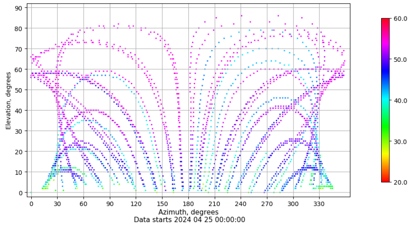
Azimuth-elevation plot for station SINE. Signal to Noise S1C Data file SINE00ESP_R_2024116.xtr
