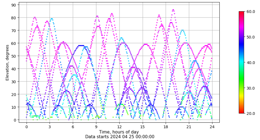
Time-elevation plot for station SINE. Signal to Noise S1C Data file SINE00ESP_R_2024116.xtr
