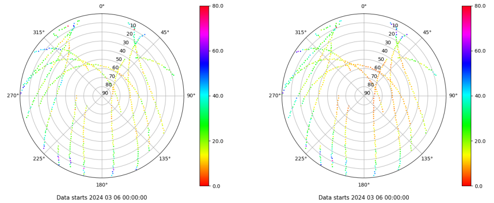
Skyplot for station SINE. Parameter M1C Data file SINE00ESP_R_2024066.xtr Skyplot for station SINE. Parameter M2P Data file SINE00ESP_R_2024066.xtr
