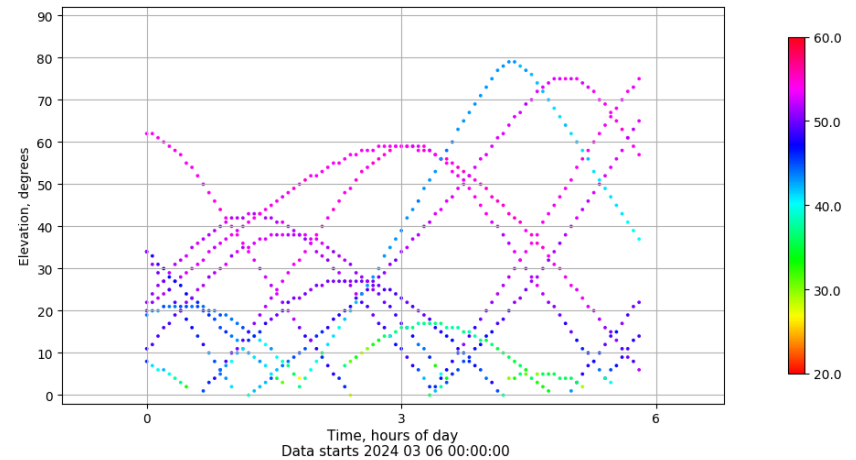
Time-elevation plot for station SINE. Signal to Noise S1C Data file SINE00ESP_R_2024066.xtr
