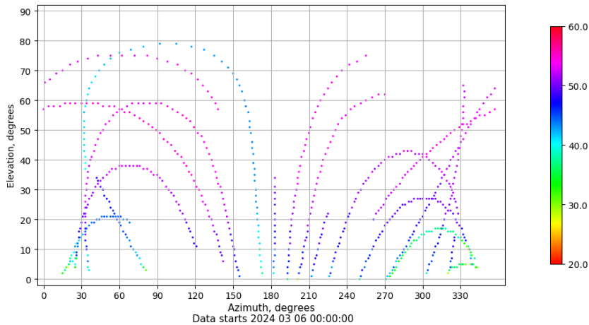
Azimuth-elevation plot for station SINE. Signal to Noise S1C Data file SINE00ESP_R_2024066.xtr
