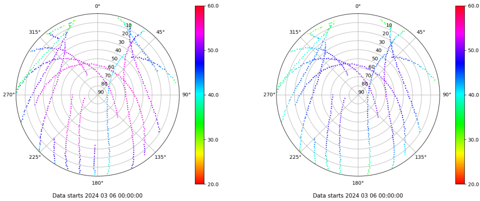
Skyplot for station SINE. Signal to Noise S1C Data file SINE00ESP_R_2024066.xtr Skyplot for station SINE. Signal to Noise S2P Data file SINE00ESP_R_2024066.xtr
