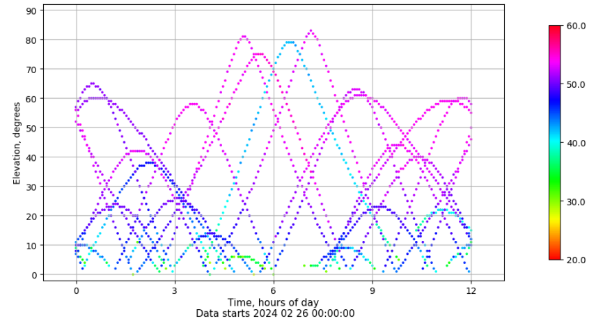
Time-elevation plot for station SINE. Signal to Noise S1C Data file SINE00ESP_R_2024057.xtr
