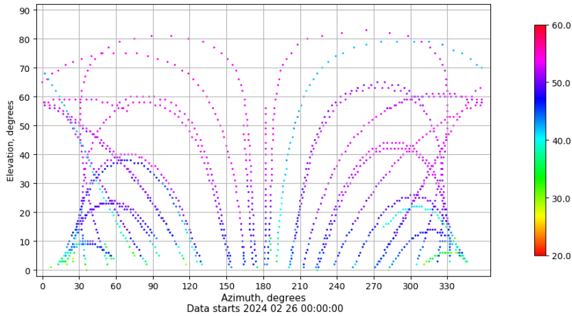
Azimuth-elevation plot for station SINE. Signal to Noise S1C Data file SINE00ESP_R_2024057.xtr
