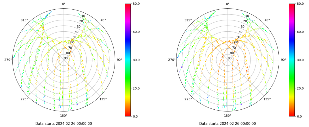
Skyplot for station SINE. Parameter M1C Data file SINE00ESP_R_2024057.xtr Skyplot for station SINE. Parameter M2P Data file SINE00ESP_R_2024057.xtr
