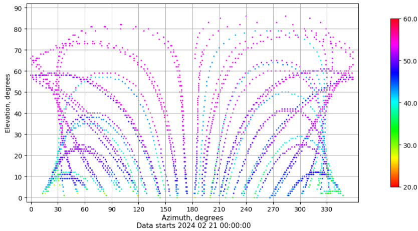
Azimuth-elevation plot for station SINE. Signal to Noise S1C Data file SINE00ESP_R_2024052.xtr
