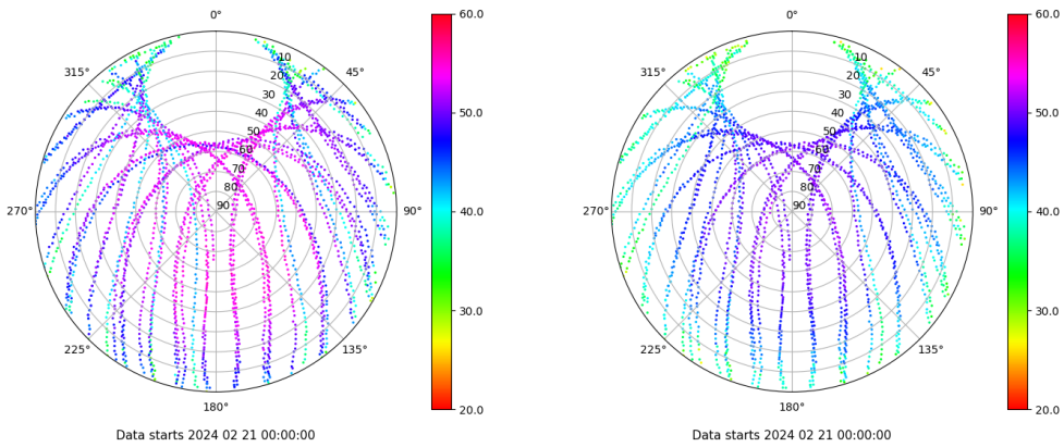
Skyplot for station SINE. Signal to Noise S1C Data file SINE00ESP_R_2024052.xtr Skyplot for station SINE. Signal to Noise S2P Data file SINE00ESP_R_2024052.xtr
