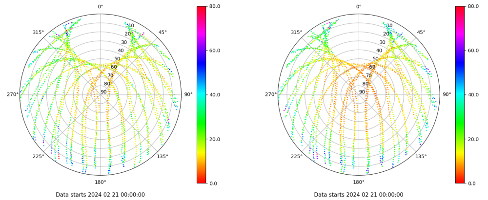
Skyplot for station SINE. Parameter M1C Data file SINE00ESP_R_2024052.xtr Skyplot for station SINE. Parameter M2P Data file SINE00ESP_R_2024052.xtr
