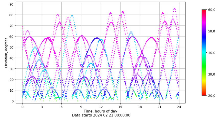
Time-elevation plot for station SINE. Signal to Noise S1C Data file SINE00ESP_R_2024052.xtr
