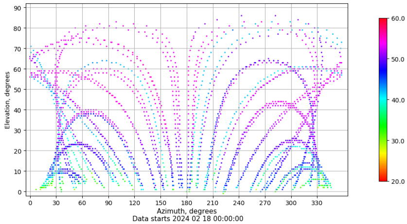
Azimuth-elevation plot for station SINE. Signal to Noise S1C Data file SINE00ESP_R_2024049.xtr
