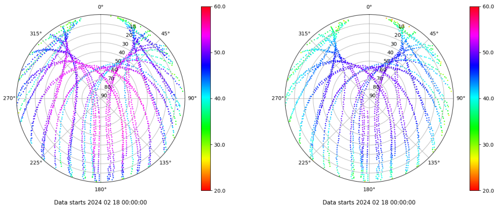
Skyplot for station SINE. Signal to Noise S1C Data file SINE00ESP_R_2024049.xtr Skyplot for station SINE. Signal to Noise S2P Data file SINE00ESP_R_2024049.xtr
