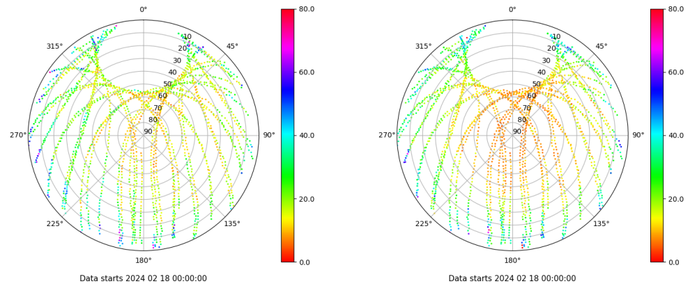
Skyplot for station SINE. Parameter M1C Data file SINE00ESP_R_2024049.xtr Skyplot for station SINE. Parameter M2P Data file SINE00ESP_R_2024049.xtr
