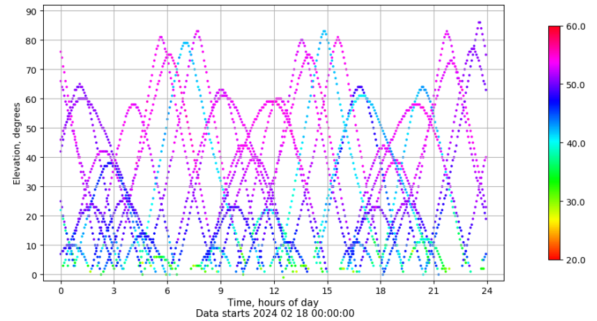
Time-elevation plot for station SINE. Signal to Noise S1C Data file SINE00ESP_R_2024049.xtr
