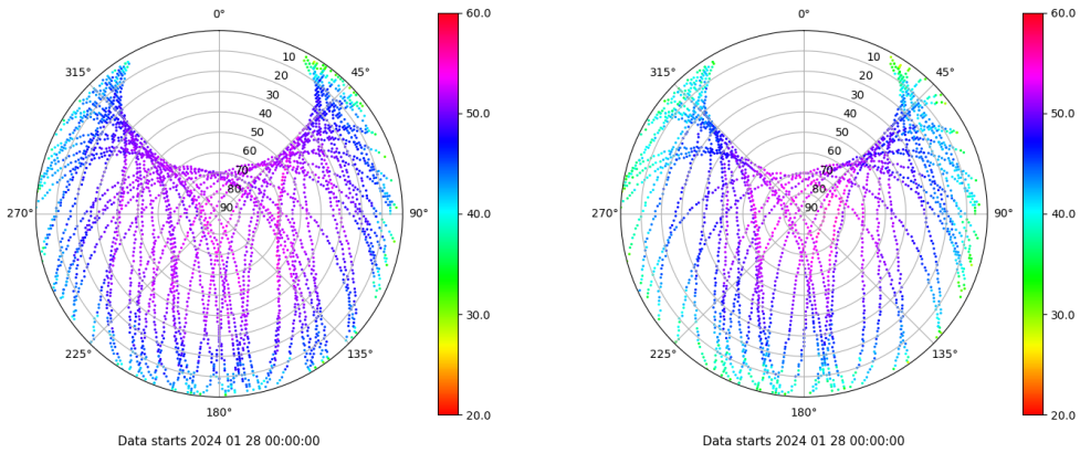
Skyplot for station SINE. Signal to Noise S1C Data file SINE00ESP_R_2024028.xtr Skyplot for station SINE. Signal to Noise S2S Data file SINE00ESP_R_2024028.xtr
