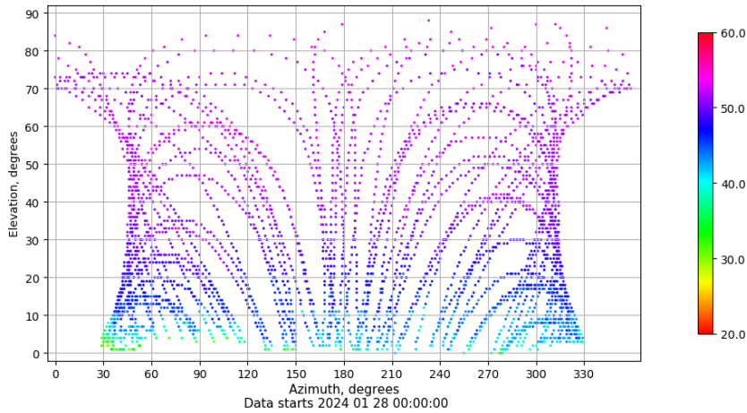
Azimuth-elevation plot for station SINE. Signal to Noise S1C Data file SINE00ESP_R_2024028.xtr
