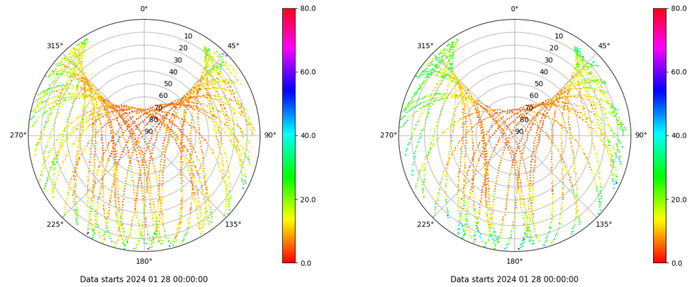
Skyplot for station SINE. Parameter M1C Data file SINE00ESP_R_2024028.xtr Skyplot for station SINE. Parameter M2S Data file SINE00ESP_R_2024028.xtr
