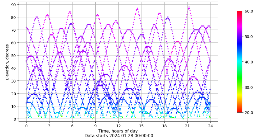
Time-elevation plot for station SINE. Signal to Noise S1C Data file SINE00ESP_R_2024028.xtr
