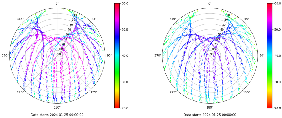
Skyplot for station SINE. Signal to Noise S1C Data file SINE00ESP_R_2024025.xtr Skyplot for station SINE. Signal to Noise S2P Data file SINE00ESP_R_2024025.xtr
