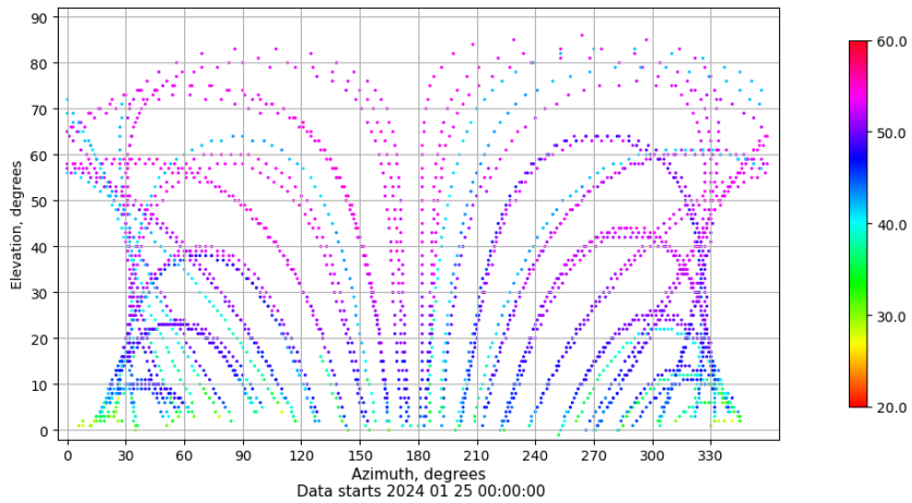
Azimuth-elevation plot for station SINE. Signal to Noise S1C Data file SINE00ESP_R_2024025.xtr
