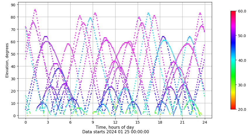
Time-elevation plot for station SINE. Signal to Noise S1C Data file SINE00ESP_R_2024025.xtr
