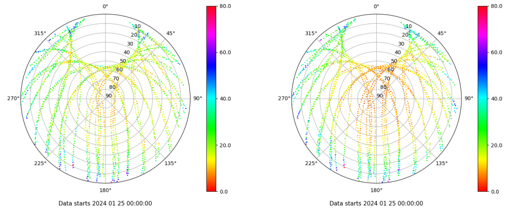
Skyplot for station SINE. Parameter M1C Data file SINE00ESP_R_2024025.xtr Skyplot for station SINE. Parameter M2P Data file SINE00ESP_R_2024025.xtr
