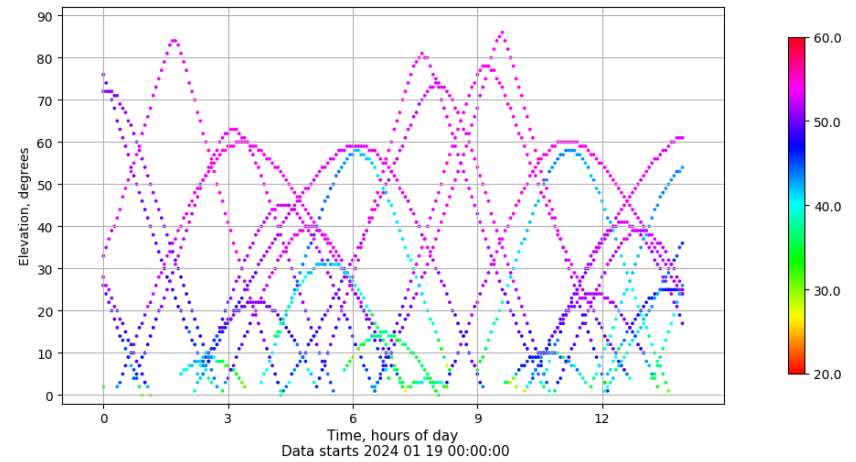
Time-elevation plot for station SINE. Signal to Noise S1C Data file SINE00ESP_R_2024019.xtr
