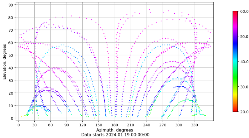
Azimuth-elevation plot for station SINE. Signal to Noise S1C Data file SINE00ESP_R_2024019.xtr
