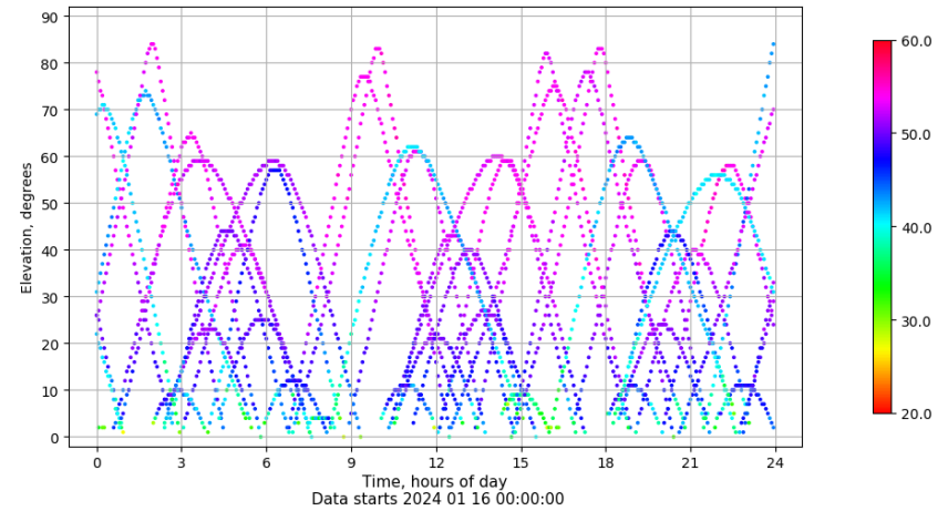
Time-elevation plot for station SINE. Signal to Noise S1C Data file SINE00ESP_R_2024016.xtr
