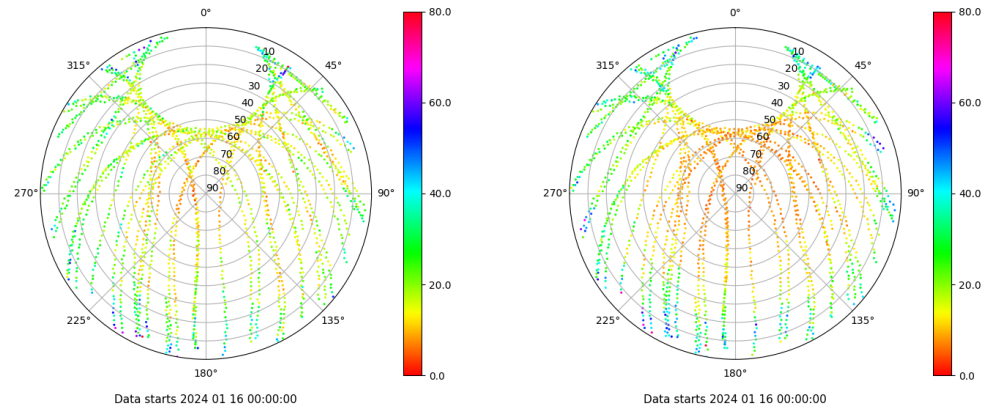
Skyplot for station SINE. Parameter M1C Data file SINE00ESP_R_2024016.xtr Skyplot for station SINE. Parameter M2P Data file SINE00ESP_R_2024016.xtr
