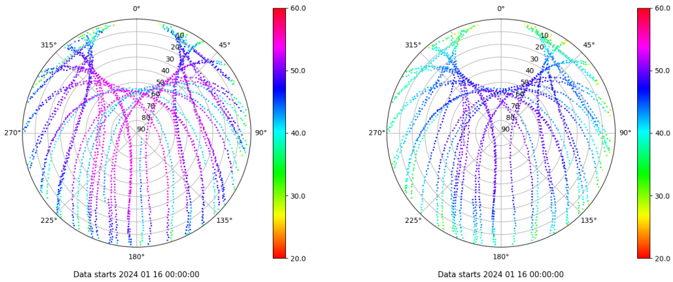
Skyplot for station SINE. Signal to Noise S1C Data file SINE00ESP_R_2024016.xtr Skyplot for station SINE. Signal to Noise S2P Data file SINE00ESP_R_2024016.xtr
