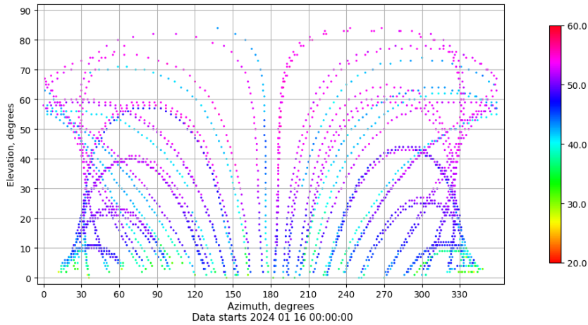
Azimuth-elevation plot for station SINE. Signal to Noise S1C Data file SINE00ESP_R_2024016.xtr
