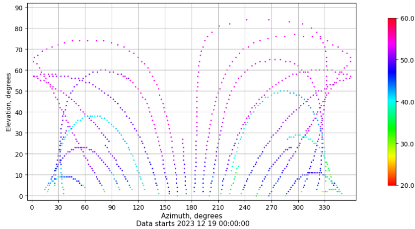
Azimuth-elevation plot for station SINE. Signal to Noise S1C Data file SINE00ESP_R_2023353.xtr
