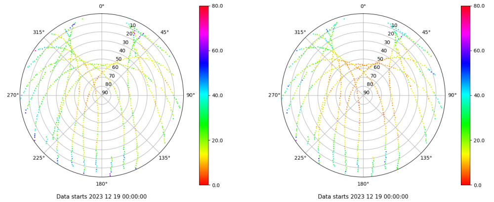
Skyplot for station SINE. Parameter M1C Data file SINE00ESP_R_2023353.xtr Skyplot for station SINE. Parameter M2P Data file SINE00ESP_R_2023353.xtr
