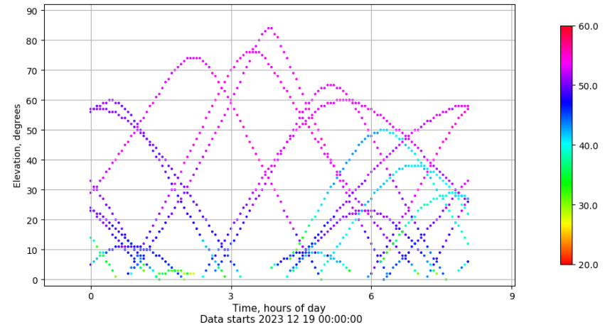
Time-elevation plot for station SINE. Signal to Noise S1C Data file SINE00ESP_R_2023353.xtr
