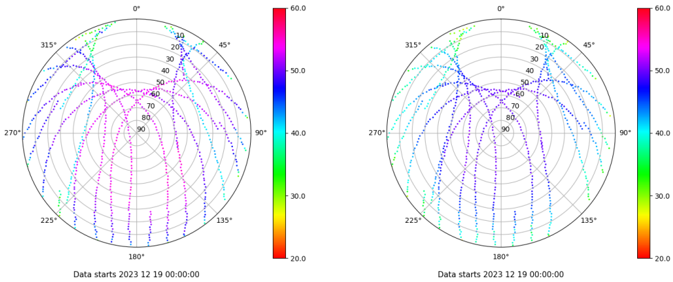
Skyplot for station SINE. Signal to Noise S1C Data file SINE00ESP_R_2023353.xtr Skyplot for station SINE. Signal to Noise S2P Data file SINE00ESP_R_2023353.xtr
