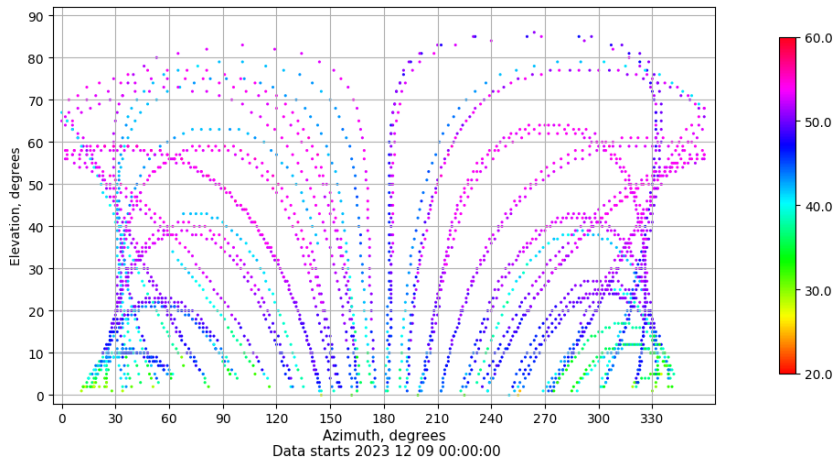
Azimuth-elevation plot for station SINE. Signal to Noise S1C Data file SINE00ESP_R_2023343.xtr
