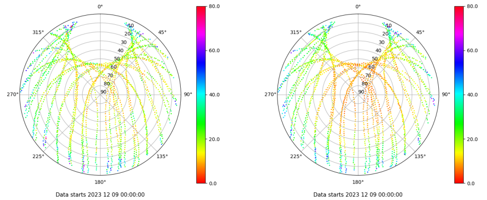
Skyplot for station SINE. Parameter M1C Data file SINE00ESP_R_2023343.xtr Skyplot for station SINE. Parameter M2P Data file SINE00ESP_R_2023343.xtr
