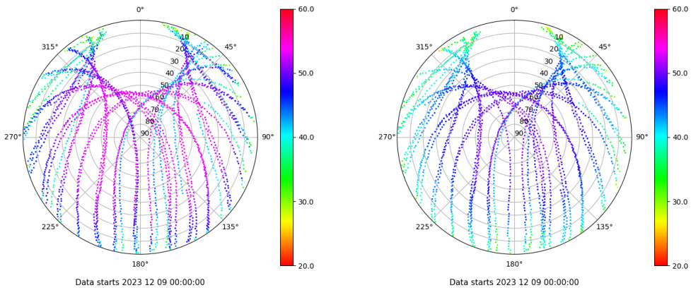
Skyplot for station SINE. Signal to Noise S1C Data file SINE00ESP_R_2023343.xtr Skyplot for station SINE. Signal to Noise S2P Data file SINE00ESP_R_2023343.xtr
