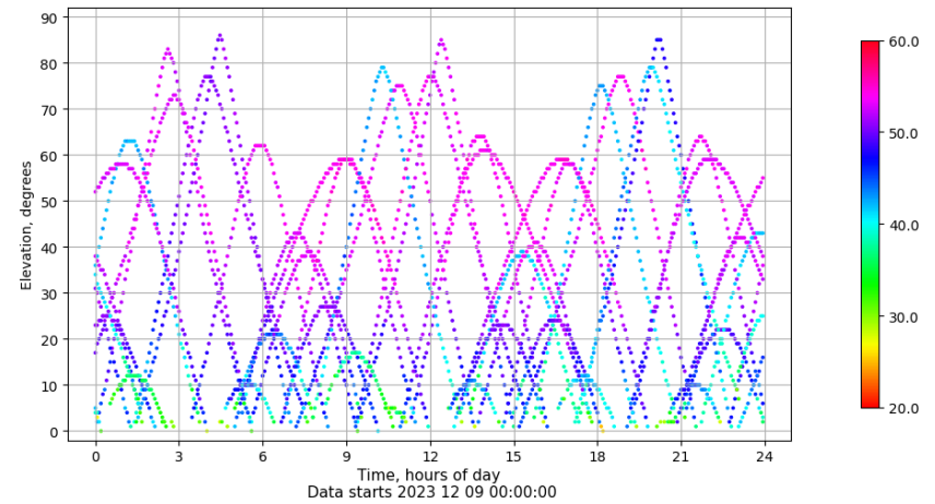
Time-elevation plot for station SINE. Signal to Noise S1C Data file SINE00ESP_R_2023343.xtr
