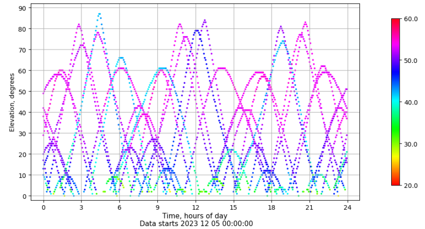
Time-elevation plot for station SINE. Signal to Noise S1C Data file SINE00ESP_R_20233339.xtr
