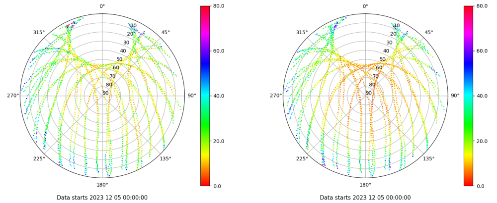
Skyplot for station SINE. Parameter M1C Data file SINE00ESP_R_20233339.xtr Skyplot for station SINE. Parameter M2P Data file SINE00ESP_R_20233339.xtr
