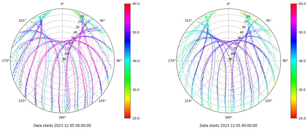
Skyplot for station SINE. Signal to Noise S1C Data file SINE00ESP_R_20233339.xtr Skyplot for station SINE. Signal to Noise S2P Data file SINE00ESP_R_20233339.xtr
