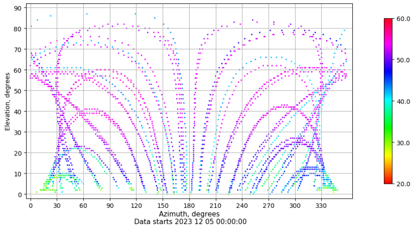
Azimuth-elevation plot for station SINE. Signal to Noise S1C Data file SINE00ESP_R_20233339.xtr
