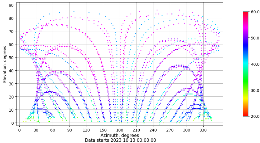
Azimuth-elevation plot for station SINE. Signal to Noise S1C Data file SINE00ESP_R_2023286.xtr
