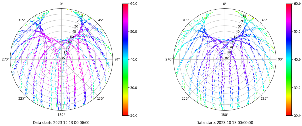
Skyplot for station SINE. Signal to Noise S1C Data file SINE00ESP_R_2023286.xtr Skyplot for station SINE. Signal to Noise S2P Data file SINE00ESP_R_2023286.xtr
