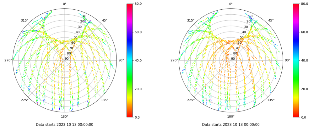
Skyplot for station SINE. Parameter M1C Data file SINE00ESP_R_2023286.xtr Skyplot for station SINE. Parameter M2P Data file SINE00ESP_R_2023286.xtr
