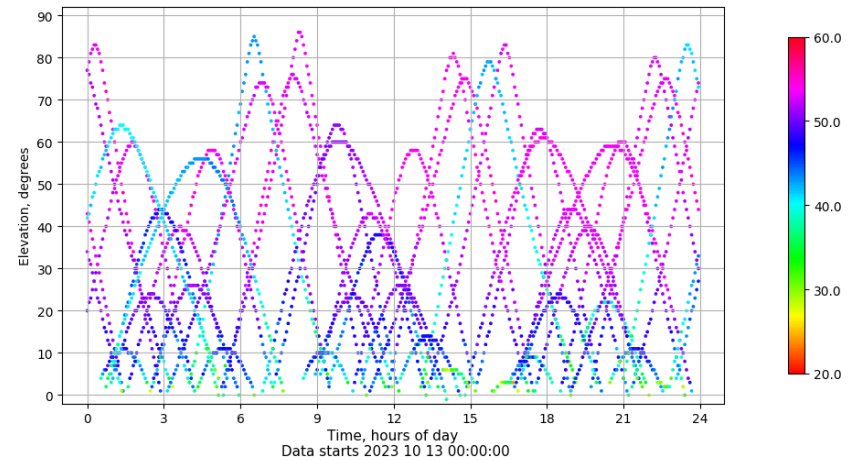
Time-elevation plot for station SINE. Signal to Noise S1C Data file SINE00ESP_R_2023286.xtr
