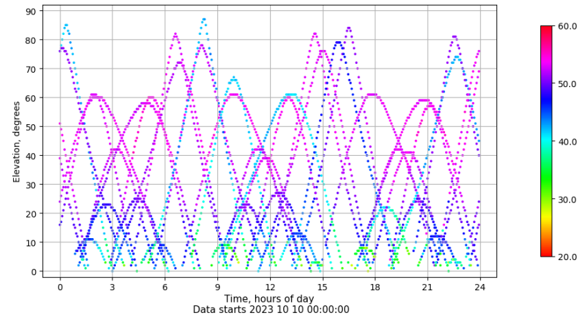
Time-elevation plot for station SINE. Signal to Noise S1C Data file SINE00ESP_R_2023283.xtr
