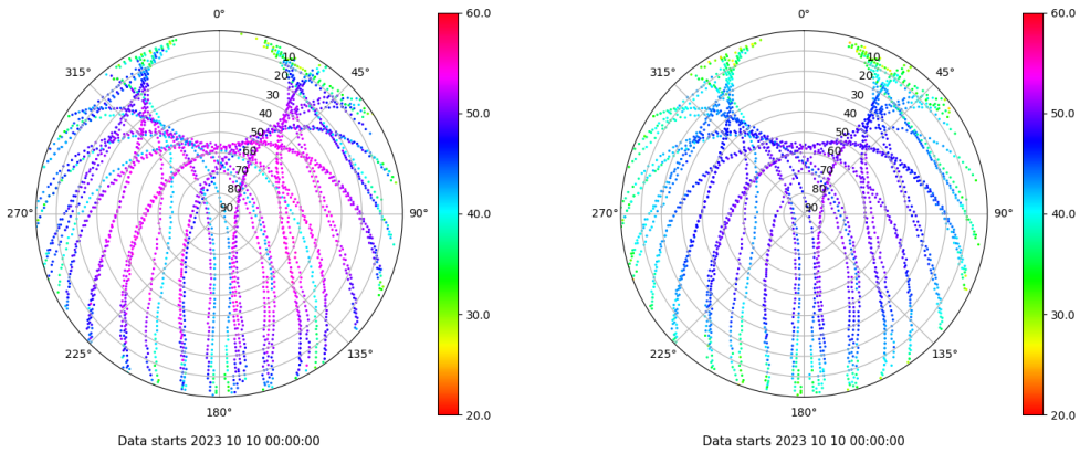
Skyplot for station SINE. Signal to Noise S1C Data file SINE00ESP_R_2023283.xtr Skyplot for station SINE. Signal to Noise S2P Data file SINE00ESP_R_2023283.xtr
