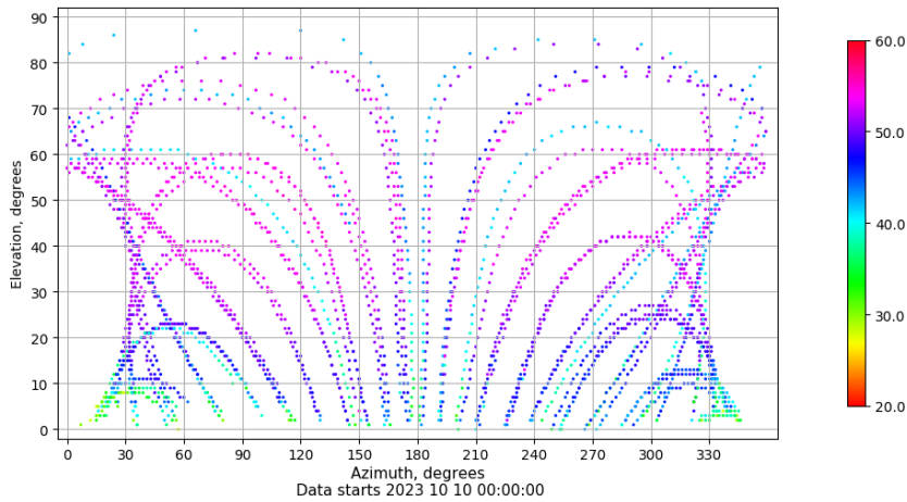
Azimuth-elevation plot for station SINE. Signal to Noise S1C Data file SINE00ESP_R_2023283.xtr
