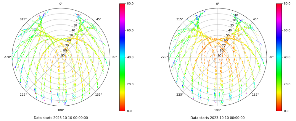
Skyplot for station SINE. Parameter M1C Data file SINE00ESP_R_2023283.xtr Skyplot for station SINE. Parameter M2P Data file SINE00ESP_R_2023283.xtr
