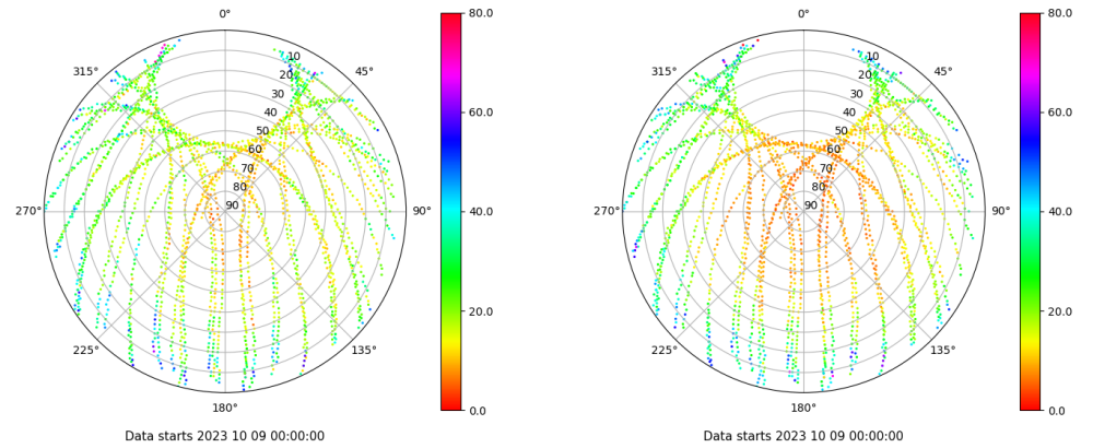
Skyplot for station SINE. Parameter M1C Data file SINE00ESP_R_2023282.xtr Skyplot for station SINE. Parameter M2P Data file SINE00ESP_R_2023282.xtr
