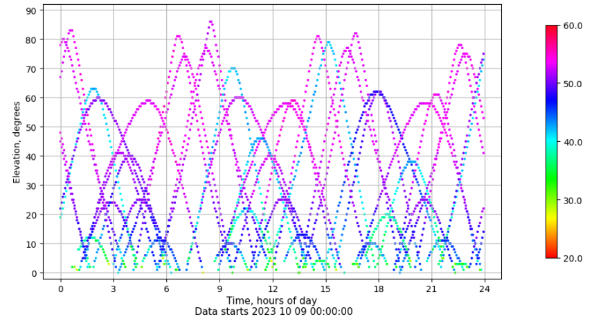
Time-elevation plot for station SINE. Signal to Noise S1C Data file SINE00ESP_R_2023282.xtr
