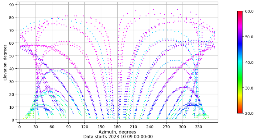
Azimuth-elevation plot for station SINE. Signal to Noise S1C Data file SINE00ESP_R_2023282.xtr
