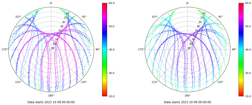
Skyplot for station SINE. Signal to Noise S1C Data file SINE00ESP_R_2023282.xtr Skyplot for station SINE. Signal to Noise S2P Data file SINE00ESP_R_2023282.xtr
