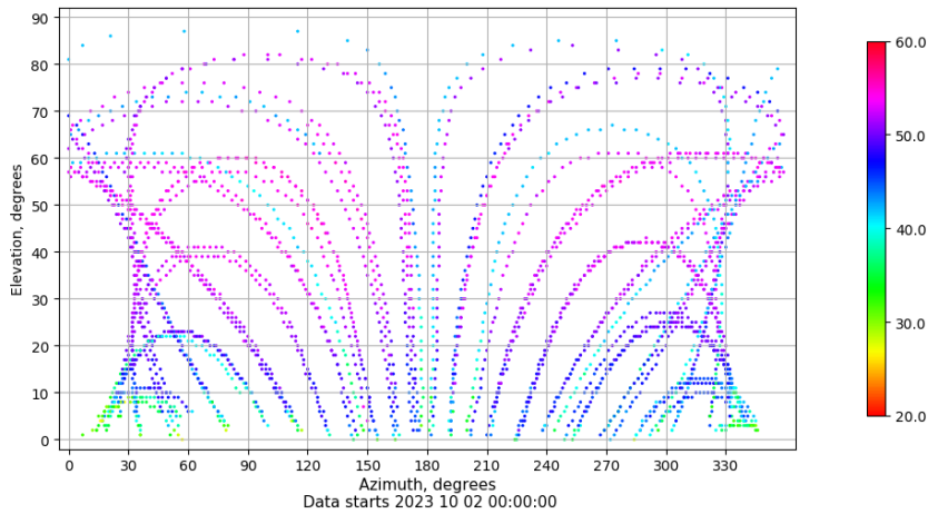
Azimuth-elevation plot for station SINE. Signal to Noise S1C Data file SINE00ESP_R_2023275.xtr
