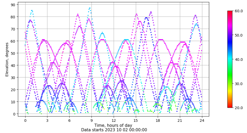
Time-elevation plot for station SINE. Signal to Noise S1C Data file SINE00ESP_R_2023275.xtr
