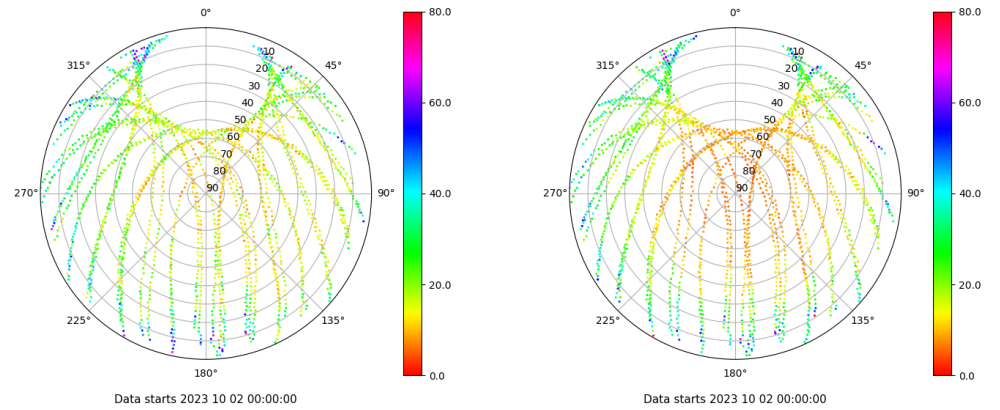
Skyplot for station SINE. Parameter M1C Data file SINE00ESP_R_2023275.xtr Skyplot for station SINE. Parameter M2P Data file SINE00ESP_R_2023275.xtr
