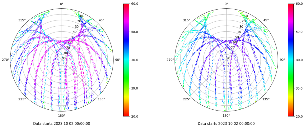
Skyplot for station SINE. Signal to Noise S1C Data file SINE00ESP_R_2023275.xtr Skyplot for station SINE. Signal to Noise S2P Data file SINE00ESP_R_2023275.xtr
