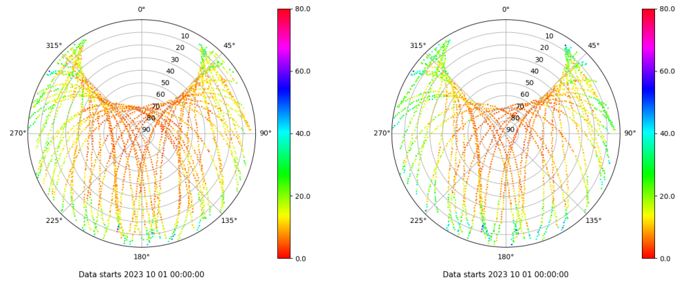
Skyplot for station SINE. Parameter M1C Data file SINE00ESP_R_2023274.xtr Skyplot for station SINE. Parameter M2S Data file SINE00ESP_R_2023274.xtr
