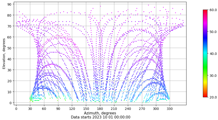
Azimuth-elevation plot for station SINE. Signal to Noise S1C Data file SINE00ESP_R_2023274.xtr
