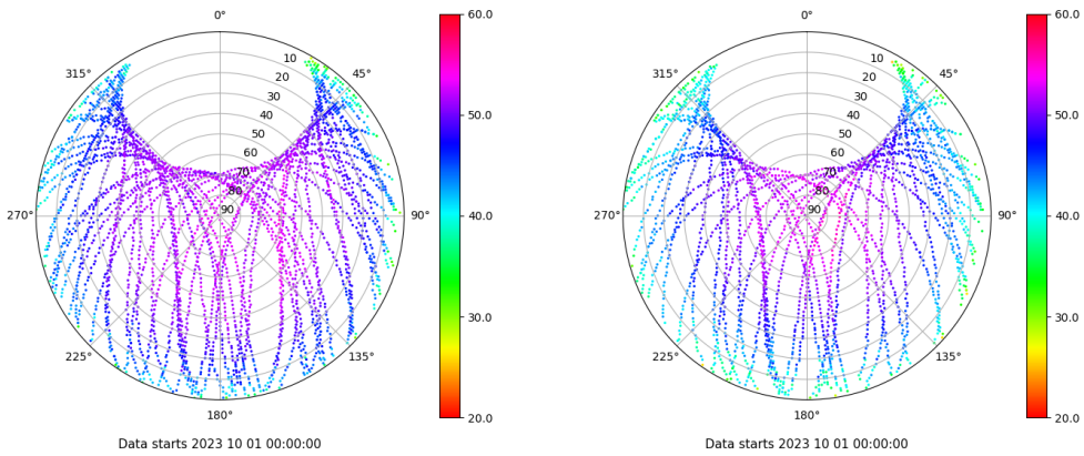
Skyplot for station SINE. Signal to Noise S1C Data file SINE00ESP_R_2023274.xtr Skyplot for station SINE. Signal to Noise S2S Data file SINE00ESP_R_2023274.xtr
