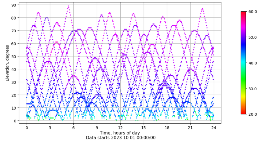
Time-elevation plot for station SINE. Signal to Noise S1C Data file SINE00ESP_R_2023274.xtr
