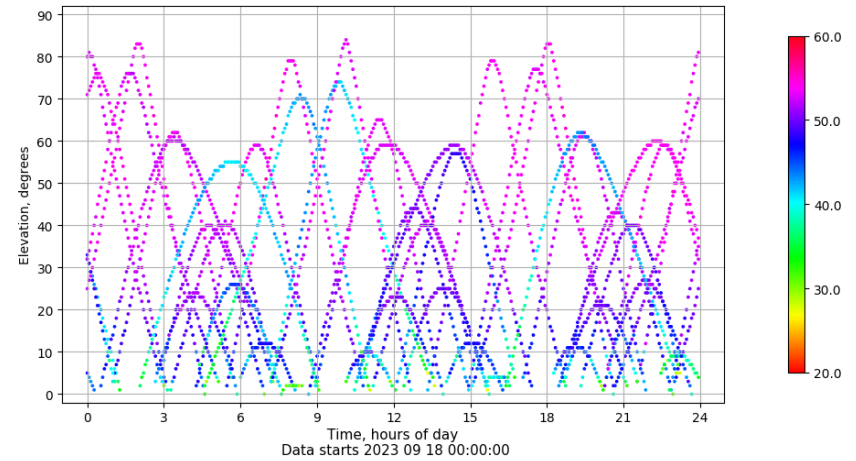
Time-elevation plot for station SINE. Signal to Noise S1C Data file SINE00ESP_R_2023261.xtr
