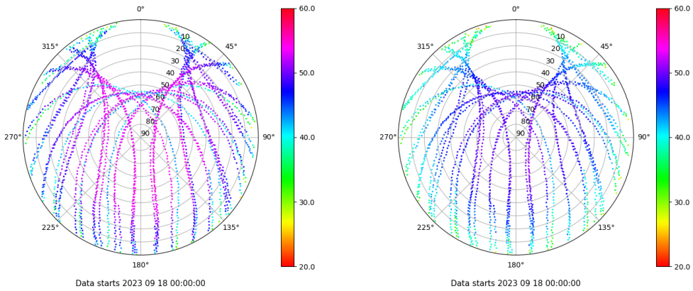
Skyplot for station SINE. Signal to Noise S1C Data file SINE00ESP_R_2023261.xtr Skyplot for station SINE. Signal to Noise S2P Data file SINE00ESP_R_2023261.xtr
