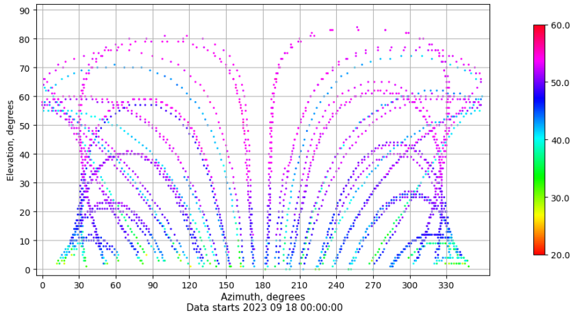
Azimuth-elevation plot for station SINE. Signal to Noise S1C Data file SINE00ESP_R_2023261.xtr
