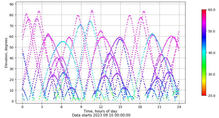
Time-elevation plot for station SINE. Signal to Noise S1C Data file SINE00ESP_R_2023253.xtr
