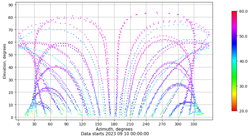
Azimuth-elevation plot for station SINE. Signal to Noise S1C Data file SINE00ESP_R_2023253.xtr
