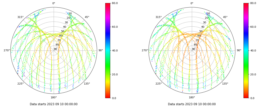
Skyplot for station SINE. Parameter M1C Data file SINE00ESP_R_2023253.xtr Skyplot for station SINE. Parameter M2P Data file SINE00ESP_R_2023253.xtr
