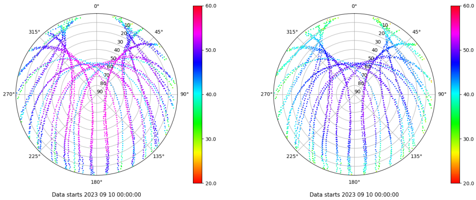
Skyplot for station SINE. Signal to Noise S1C Data file SINE00ESP_R_2023253.xtr Skyplot for station SINE. Signal to Noise S2P Data file SINE00ESP_R_2023253.xtr
