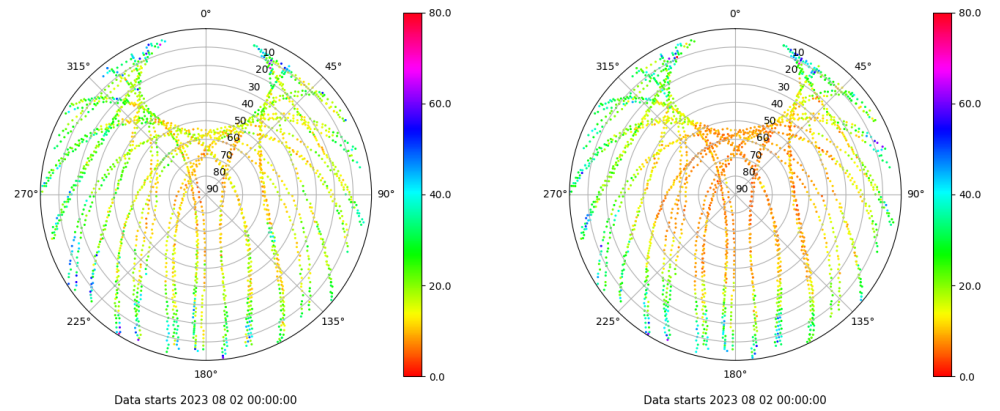
Skyplot for station SINE. Parameter M1C Data file SINE00ESP_R_2023214.xtr Skyplot for station SINE. Parameter M2P Data file SINE00ESP_R_2023214.xtr
