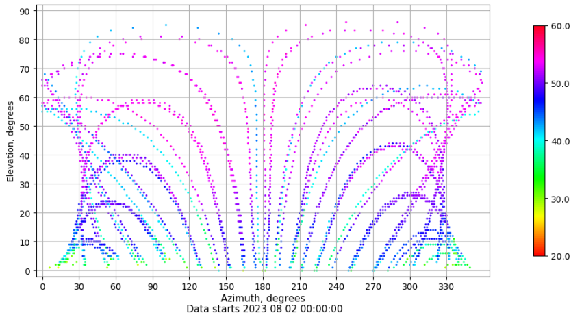
Azimuth-elevation plot for station SINE. Signal to Noise S1C Data file SINE00ESP_R_2023214.xtr
