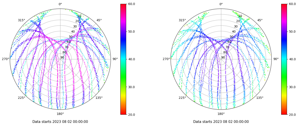
Skyplot for station SINE. Signal to Noise S1C Data file SINE00ESP_R_2023214.xtr Skyplot for station SINE. Signal to Noise S2P Data file SINE00ESP_R_2023214.xtr
