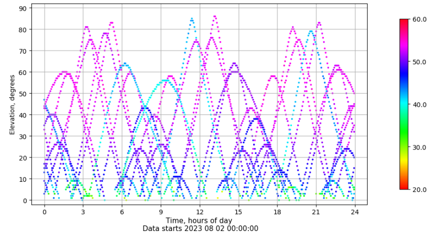
Time-elevation plot for station SINE. Signal to Noise S1C Data file SINE00ESP_R_2023214.xtr
