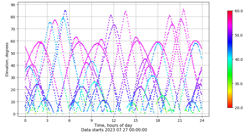
Time-elevation plot for station SINE. Signal to Noise S1C Data file SINE00ESP_R_2023208.xtr
