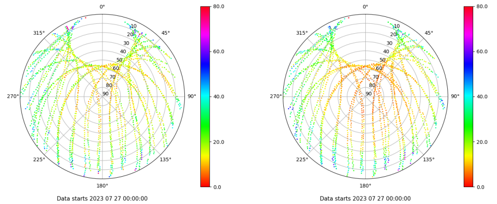
Skyplot for station SINE. Parameter M1C Data file SINE00ESP_R_2023208.xtr Skyplot for station SINE. Parameter M2P Data file SINE00ESP_R_2023208.xtr
