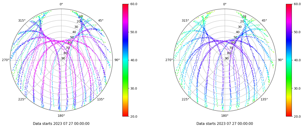
Skyplot for station SINE. Signal to Noise S1C Data file SINE00ESP_R_2023208.xtr Skyplot for station SINE. Signal to Noise S2P Data file SINE00ESP_R_2023208.xtr
