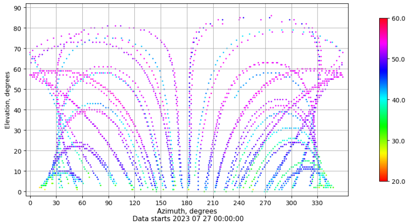
Azimuth-elevation plot for station SINE. Signal to Noise S1C Data file SINE00ESP_R_2023208.xtr
