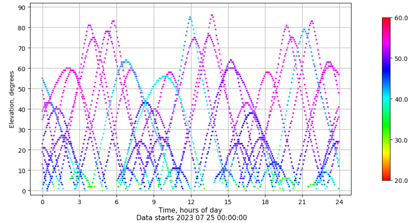
Time-elevation plot for station SINE. Signal to Noise S1C Data file SINE00ESP_R_2023206.xtr
