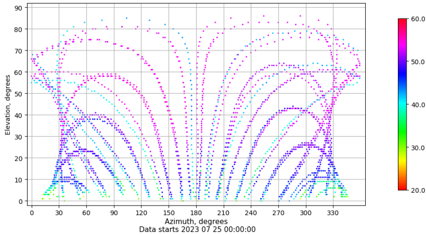
Azimuth-elevation plot for station SINE. Signal to Noise S1C Data file SINE00ESP_R_2023206.xtr
