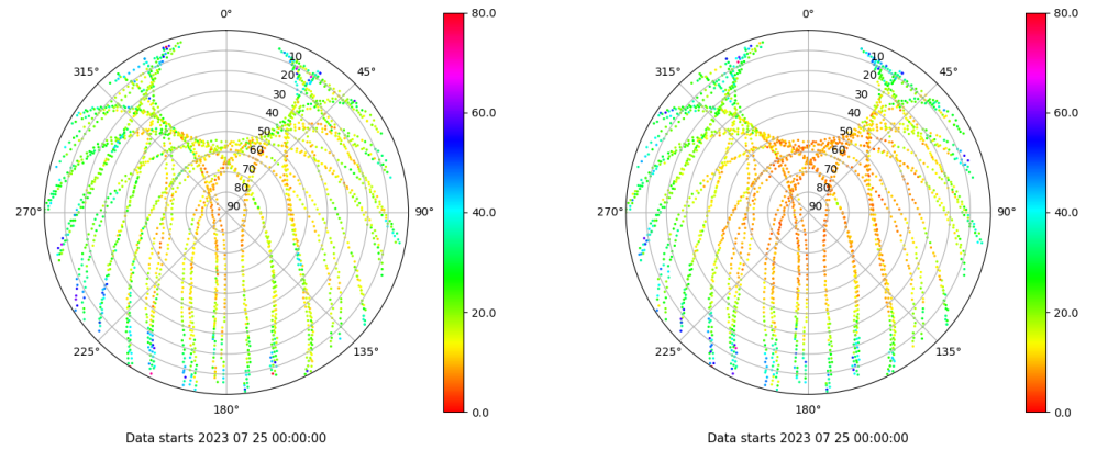
Skyplot for station SINE. Parameter M1C Data file SINE00ESP_R_2023206.xtr Skyplot for station SINE. Parameter M2P Data file SINE00ESP_R_2023206.xtr
