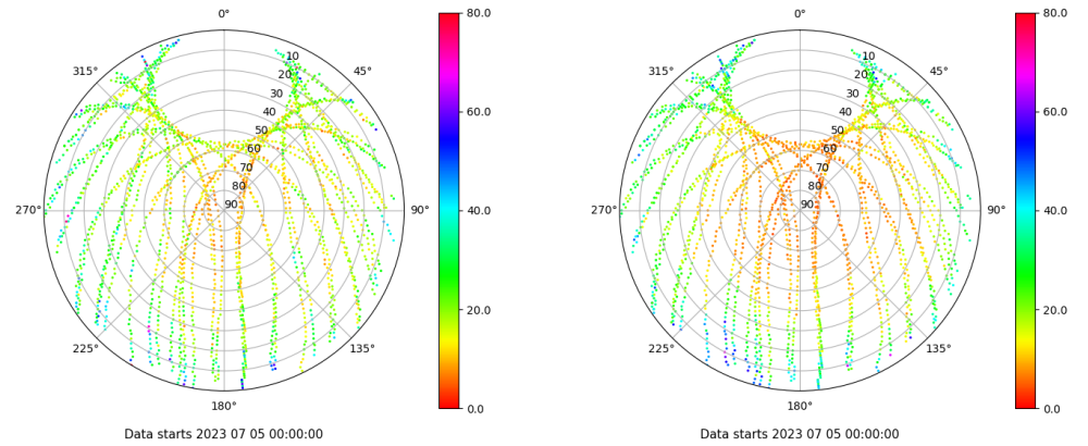
Skyplot for station SINE. Parameter M1C Data file SINE00ESP_R_2023186.xtr Skyplot for station SINE. Parameter M2P Data file SINE00ESP_R_2023186.xtr
