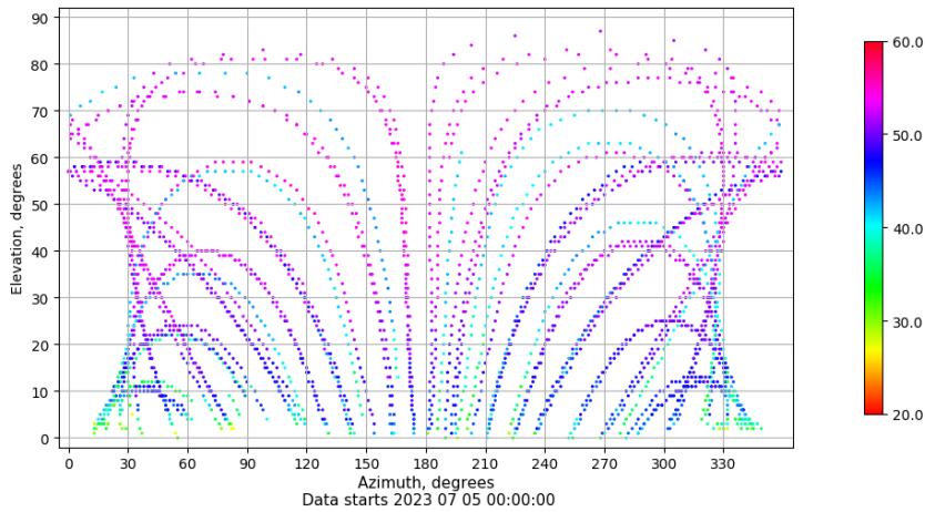
Azimuth-elevation plot for station SINE. Signal to Noise S1C Data file SINE00ESP_R_2023186.xtr
