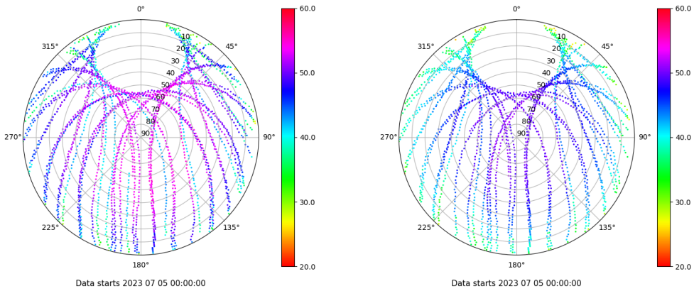
Skyplot for station SINE. Signal to Noise S1C Data file SINE00ESP_R_2023186.xtr Skyplot for station SINE. Signal to Noise S2P Data file SINE00ESP_R_2023186.xtr
