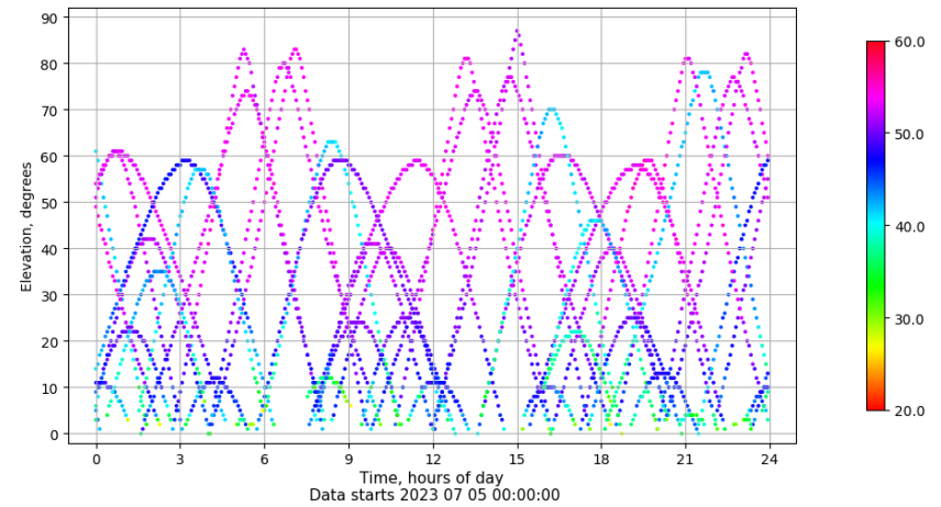
Time-elevation plot for station SINE. Signal to Noise S1C Data file SINE00ESP_R_2023186.xtr
