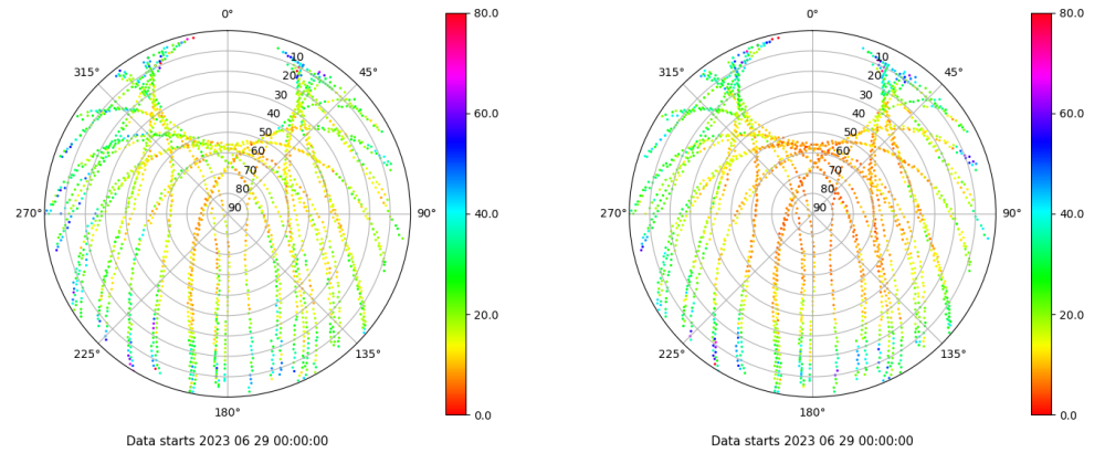
Skyplot for station SINE. Parameter M1C Data file SINE00ESP_R_2023180.xtr Skyplot for station SINE. Parameter M2P Data file SINE00ESP_R_2023180.xtr
