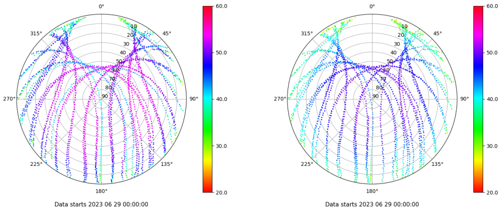
Skyplot for station SINE. Signal to Noise S1C Data file SINE00ESP_R_2023180.xtr Skyplot for station SINE. Signal to Noise S2P Data file SINE00ESP_R_2023180.xtr
