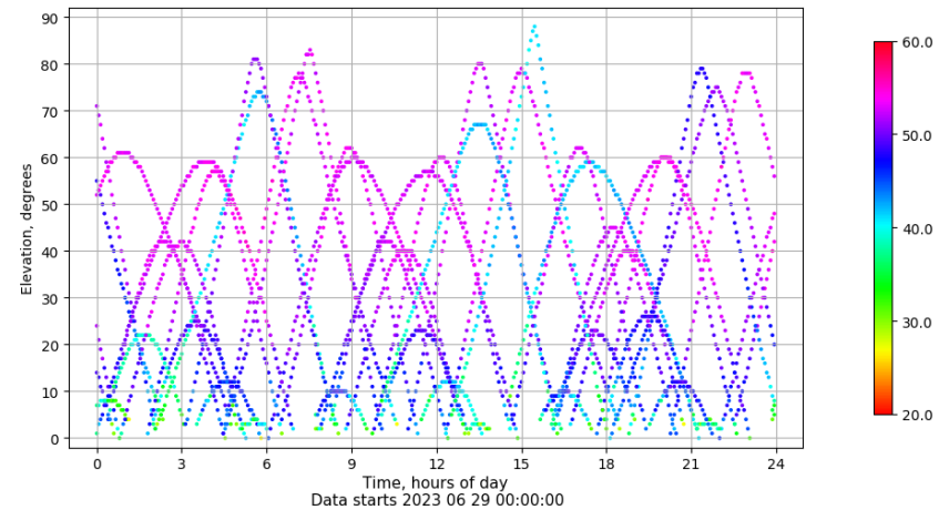
Time-elevation plot for station SINE. Signal to Noise S1C Data file SINE00ESP_R_2023180.xtr
