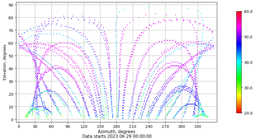
Azimuth-elevation plot for station SINE. Signal to Noise S1C Data file SINE00ESP_R_2023180.xtr
