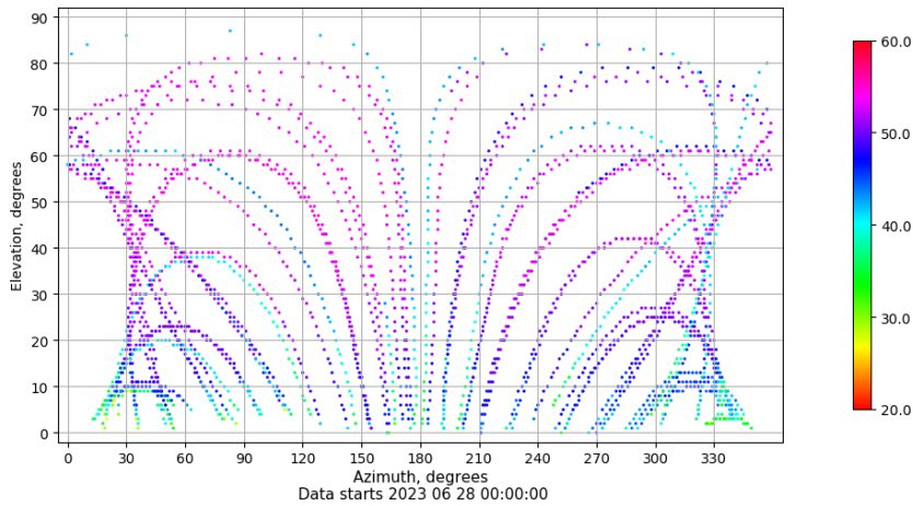
Azimuth-elevation plot for station SINE. Signal to Noise S1C Data file SINE00ESP_R_2023179.xtr
