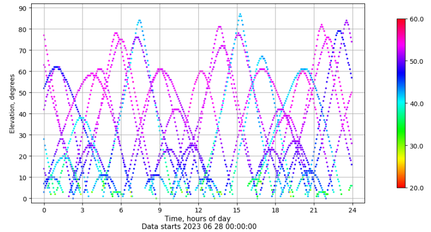
Time-elevation plot for station SINE. Signal to Noise S1C Data file SINE00ESP_R_2023179.xtr
