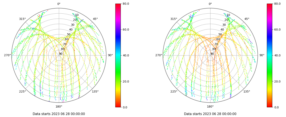
Skyplot for station SINE. Parameter M1C Data file SINE00ESP_R_2023179.xtr Skyplot for station SINE. Parameter M2P Data file SINE00ESP_R_2023179.xtr
