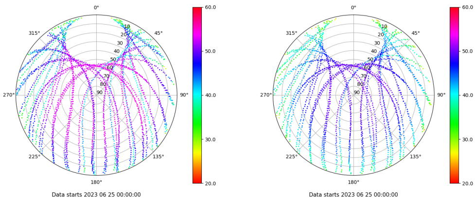
Skyplot for station SINE. Signal to Noise S1C Data file SINE00ESP_R_2023176.xtr Skyplot for station SINE. Signal to Noise S2P Data file SINE00ESP_R_2023176.xtr
