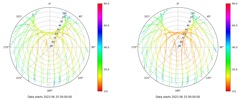
Skyplot for station SINE. Parameter M1C Data file SINE00ESP_R_2023176.xtr Skyplot for station SINE. Parameter M2P Data file SINE00ESP_R_2023176.xtr
