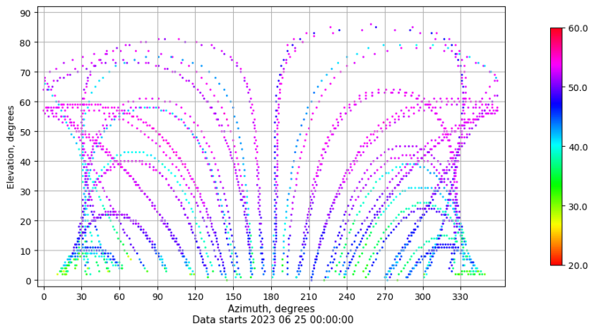
Azimuth-elevation plot for station SINE. Signal to Noise S1C Data file SINE00ESP_R_2023176.xtr
