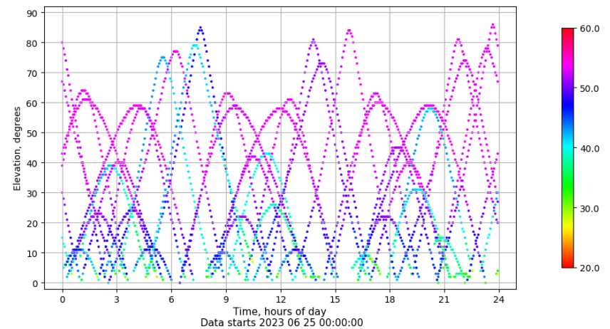
Time-elevation plot for station SINE. Signal to Noise S1C Data file SINE00ESP_R_2023176.xtr
