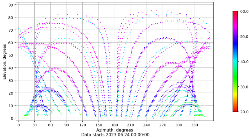
Azimuth-elevation plot for station SINE. Signal to Noise S1C Data file SINE00ESP_R_2023175.xtr
