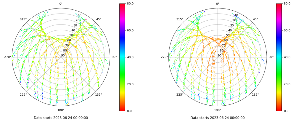
Skyplot for station SINE. Parameter M1C Data file SINE00ESP_R_2023175.xtr Skyplot for station SINE. Parameter M2P Data file SINE00ESP_R_2023175.xtr
