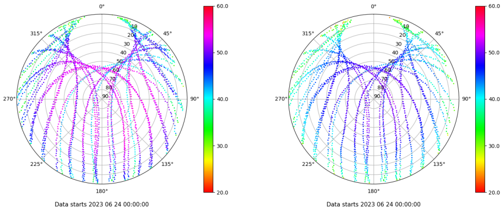
Skyplot for station SINE. Signal to Noise S1C Data file SINE00ESP_R_2023175.xtr Skyplot for station SINE. Signal to Noise S2P Data file SINE00ESP_R_2023175.xtr
