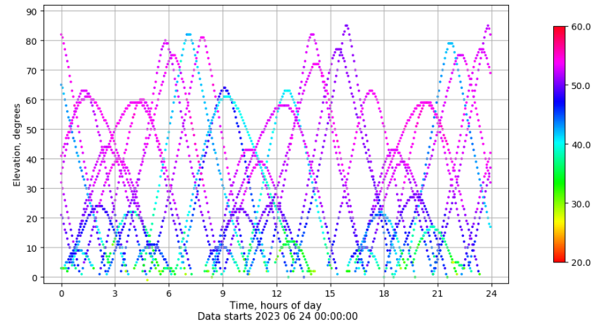
Time-elevation plot for station SINE. Signal to Noise S1C Data file SINE00ESP_R_2023175.xtr
