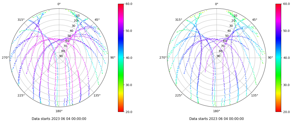
Skyplot for station SINE. Signal to Noise S1C Data file SINE00ESP_R_2023155.xtr Skyplot for station SINE. Signal to Noise S2P Data file SINE00ESP_R_2023155.xtr
