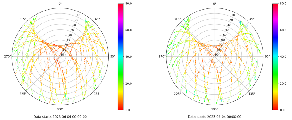
Skyplot for station SINE. Parameter M1C Data file SINE00ESP_R_2023155.xtr Skyplot for station SINE. Parameter M2S Data file SINE00ESP_R_2023155.xtr
