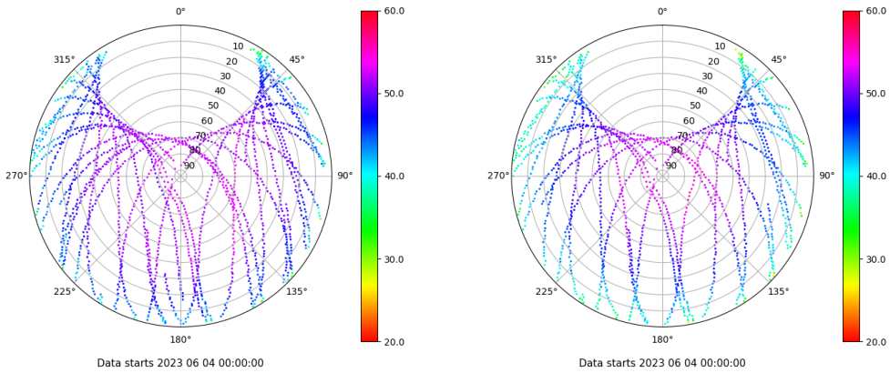
Skyplot for station SINE. Signal to Noise S1C Data file SINE00ESP_R_2023155.xtr Skyplot for station SINE. Signal to Noise S2S Data file SINE00ESP_R_2023155.xtr
