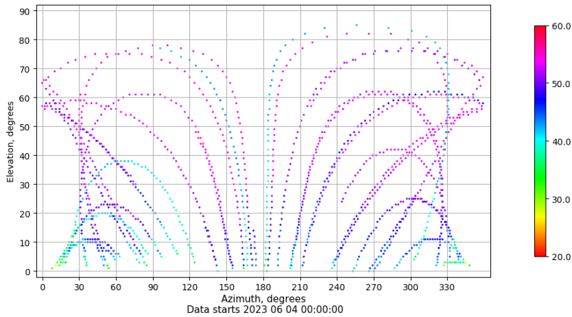
Azimuth-elevation plot for station SINE. Signal to Noise S1C Data file SINE00ESP_R_2023155.xtr
