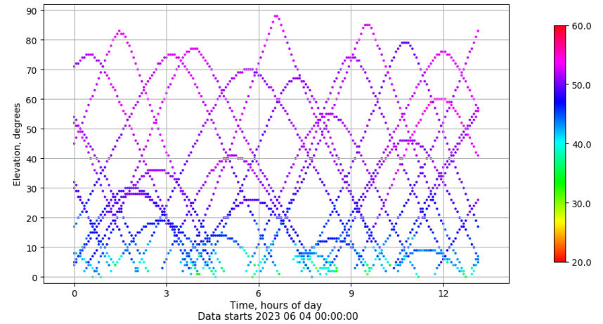
Time-elevation plot for station SINE. Signal to Noise S1C Data file SINE00ESP_R_2023155.xtr
