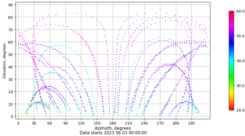
Azimuth-elevation plot for station SINE. Signal to Noise S1C Data file SINE00ESP_R_2023154.xtr
