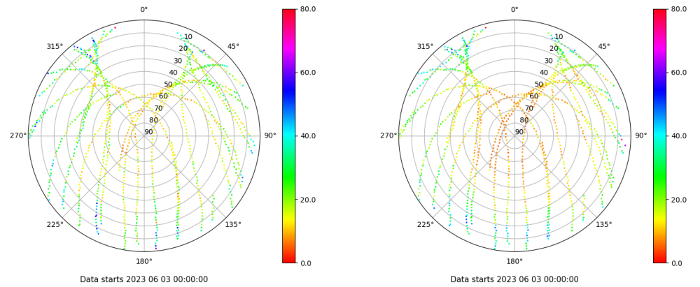
Skyplot for station SINE. Parameter M1C Data file SINE00ESP_R_2023154.xtr Skyplot for station SINE. Parameter M2P Data file SINE00ESP_R_2023154.xtr
