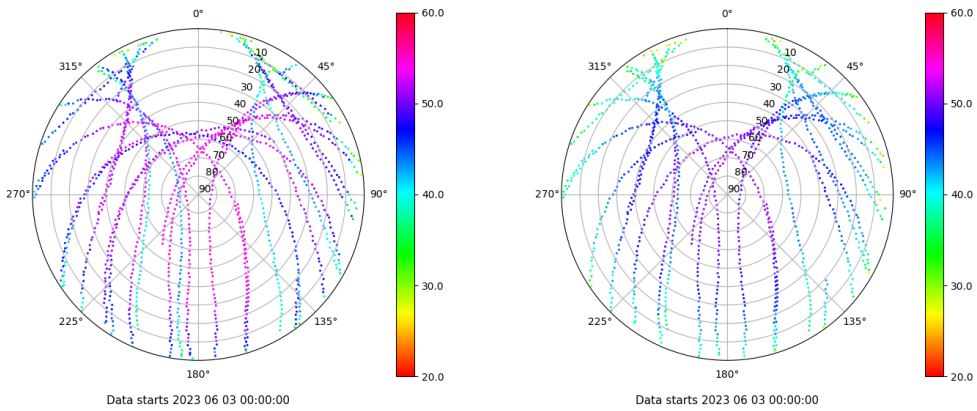
Skyplot for station SINE. Signal to Noise S1C Data file SINE00ESP_R_2023154.xtr Skyplot for station SINE. Signal to Noise S2P Data file SINE00ESP_R_2023154.xtr
