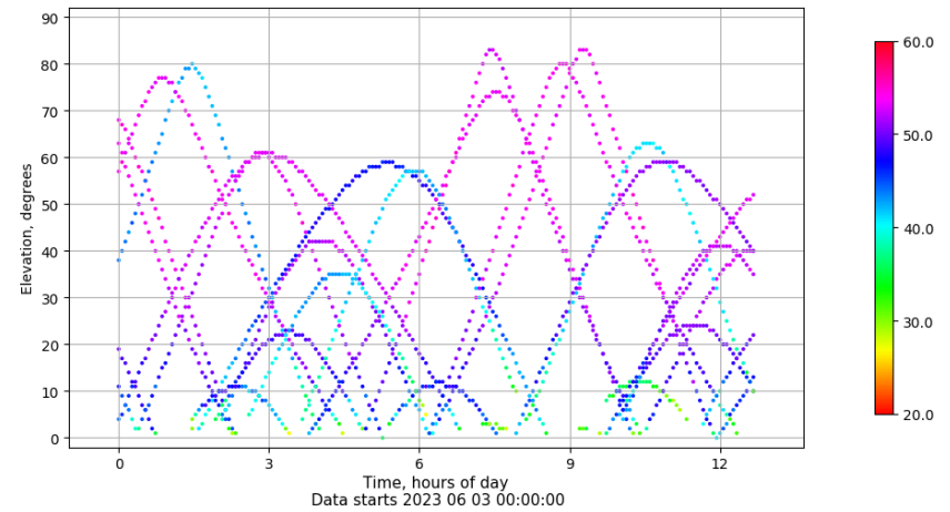
Time-elevation plot for station SINE. Signal to Noise S1C Data file SINE00ESP_R_2023154.xtr
